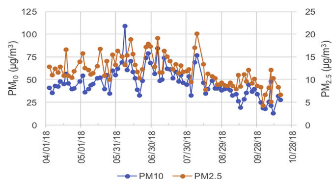
Fig. 3. Average PM 2.5 and PM 10 mass concentrations in the city of Barranquilla between April–October 2018.
