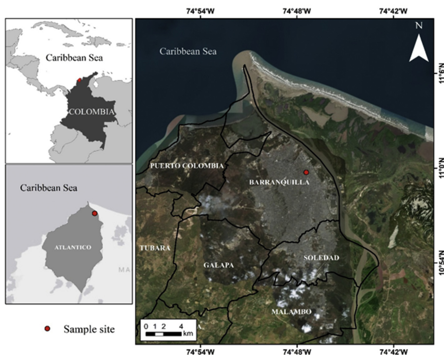
Fig. 1. Selected study area.
