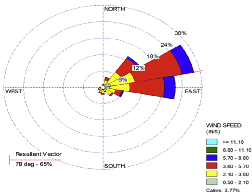
Fig. 2. Wind Rose for the period between April–October 2018.
