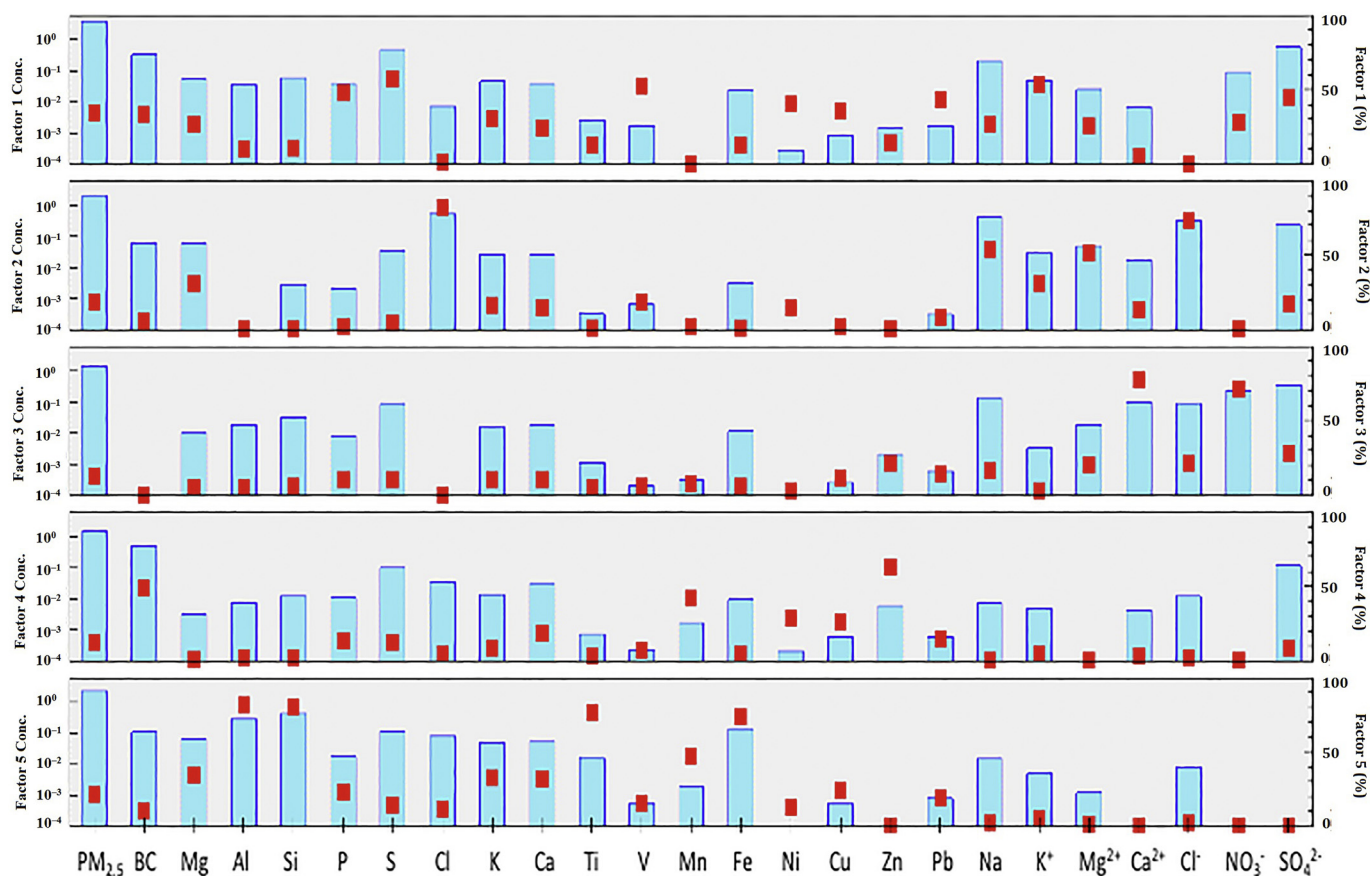
Fig. 5. Source profiles identified for the PM_{2.5} mass samples of each species assigned to the factor (blue bar, left axis) and the percentage of each species associated with the factor (red square, right axis).
