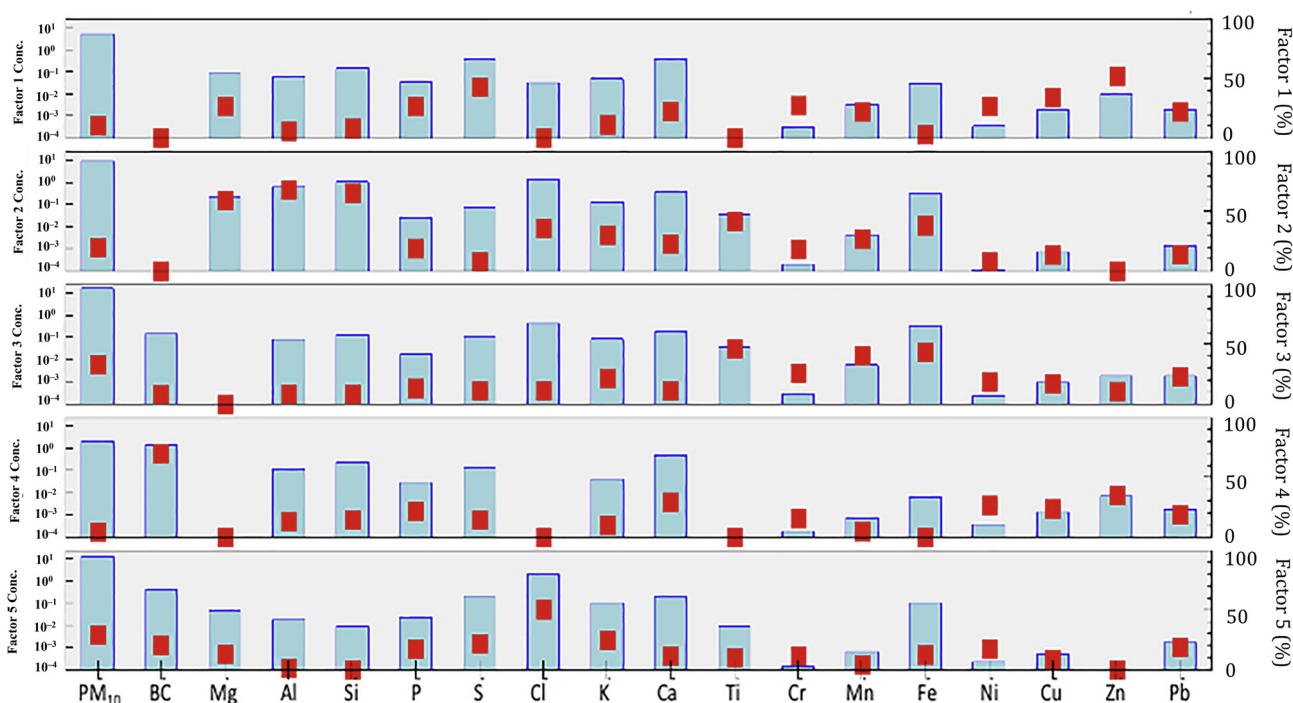
Fig. 6. Source profiles identified for the \text{PM}_{10} mass samples of each species assigned to the factor (blue bar, left axis) and the percentage of each species associated with the factor (red square, right axis).
