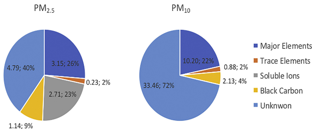
Fig. 4. Mass closure of particulate matter ( PM_{10} y PM_{2.5} ).
