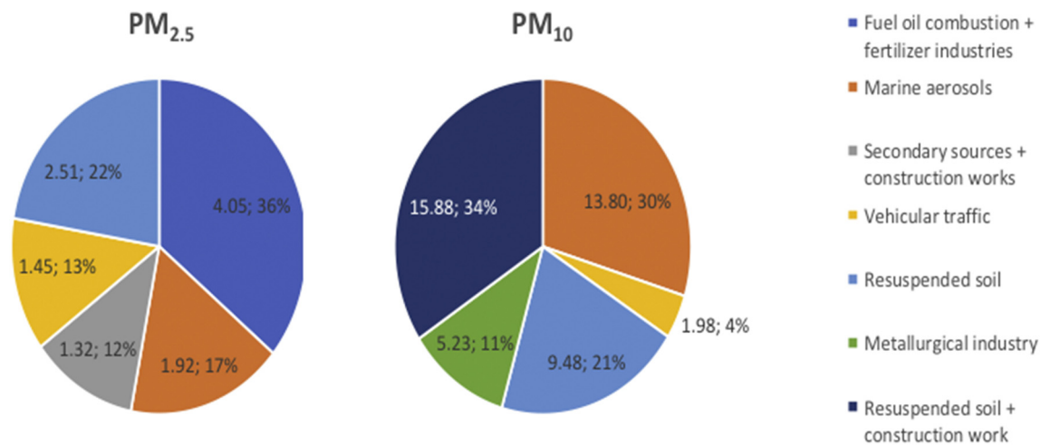
Fig. 7. Source apportionment to PM 2.5 and PM 10 mass concentrations (µg/m³).
