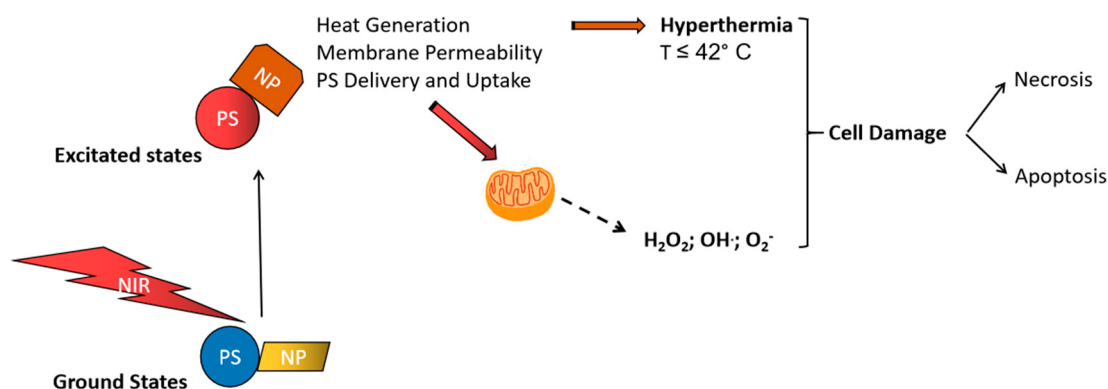
Figure 3. In combination therapy, both photodynamic and photothermal therapy (PTT) and photodynamic therapy (PDT) agents are irradiated and excited to an upper electronic level, where the PTT agent generates heat that facilitates cell membrane permeability and more PDT agent release and uptake into tumor tissue. Hyperthermia and free radical generation cause ablation and tumor damage and killing through necrosis and/or apoptosis. PS: photosensitizing molecule, NP: nanoparticle; NIR: near-infrared region.
