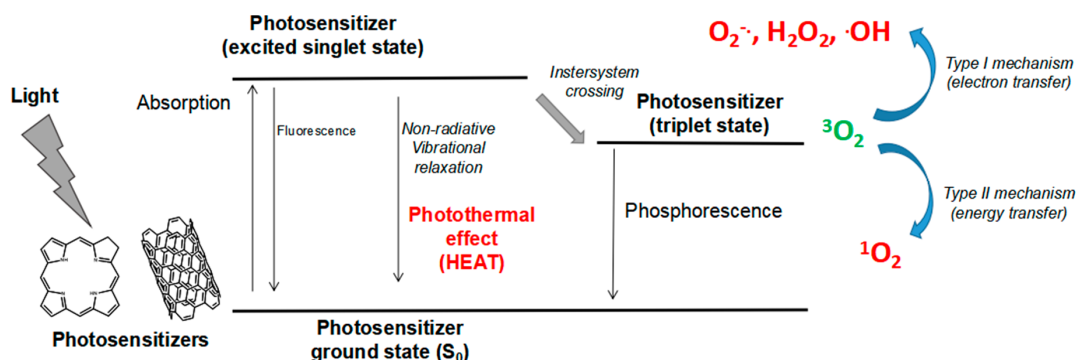
Figure 2. Simplified Jablonski diagram depicting the different energy levels induced after light irradiation. The phototherapeutic agent (photosensitizer) is excited from ground level (S 0 ) to the singlet excited state, where it may lose its absorbed energy through fluorescence or non-radiative reactions. Effective agents undergo intersystem crossing and conversion into the triplet excited state, which enables photoreactions to take place [24].
