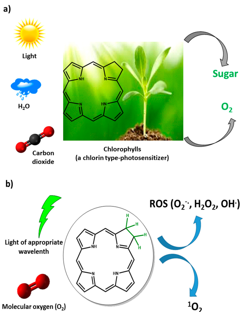
Figure 1. (a) General photosynthesis process; (b) Representation of a simple photodynamic therapy protocol. ROS: reactive oxygen species.
