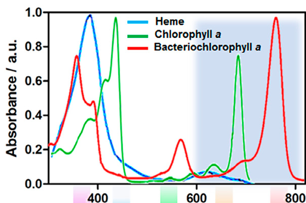
Figure 5. UV-vis absorption spectra of tetrapyrrolic macrocycles that are involved in natural processes. Reprinted from Pucelik et al. [8] with permission (open access) from Elsevier, Copyright 2020.
