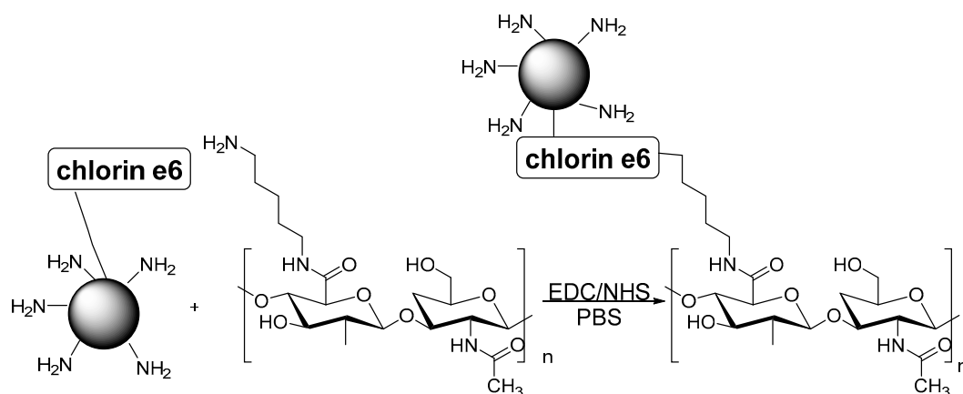
Figure 9. Bioconjugation of a chlorin-e6-functionalized carbon dot and diaminohexane-modified hyaluronate via the 1-ethyl-3-(3-dimethylaminopropyl)carbodiimide- N -hydroxysulfosuccinimide sodium (EDC-NHS) methodology.
