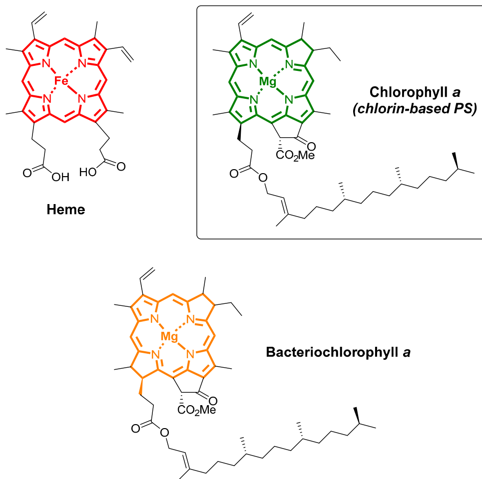
Figure 4. Tetrapyrrolic macrocycles that are involved in natural processes.
