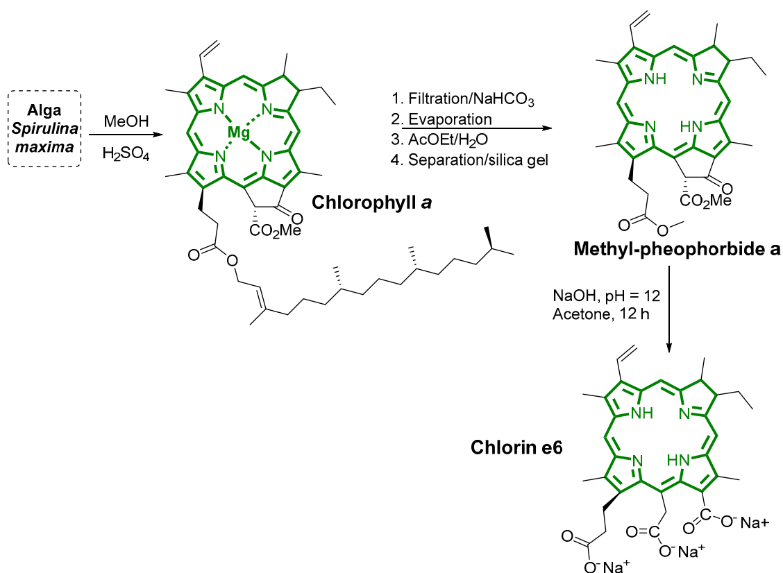
Figure 6. Methodology for the chlorin e6 extraction from Spirulina maxima .
