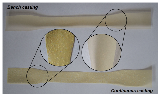
Fig. 5. Non-scaled-up and scaled-up biocomposites. Biocomposites based on carrot minimal processing waste produced on a laboratory (top) or a pilot scale (bottom).
