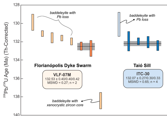
Fig. 6. Rank-order plot of U-Pb baddeleyite ages from high-Ti-Sr mafic intrusive rocks from the Paraná LIP in Brazil: a composite dyke (sample VLF-07 M – Florianópolis Dyke Swarm) and a dolerite sill (sample ITC-30 – Taió Sill) emplaced in Permian-Triassic sedimentary rocks from the Paraná basin. Vertical bars represent single grain ^{206}\text{Pb}/^{238}\text{U} baddeleyite ages with 2\sigma uncertainties. Dark colored analyses are used to calculate a weighted average age (horizontal gray bar), that represent the emplacement ages of dyke and sill. Light colored analyses were discarded from weighted average age calculations due to suspected secondary Pb-loss (younger dates) and mixture of baddeleyite with a xenocrystic zircon component (older date).
