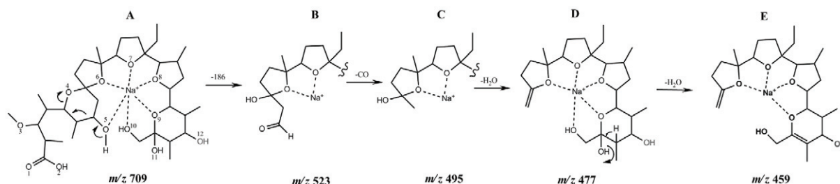
Scheme 1. The proposed fragmentation route showing the formation of product ion m/z 459 in the positive ion ESI-MS/MS of the hydroxylated metabolite of monensin A.
