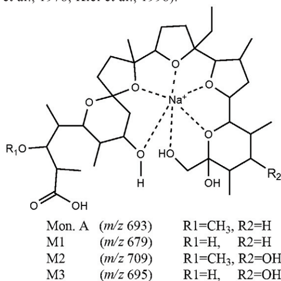
Figure 1. Monensin A and the main metabolites found in in vivo systems.
