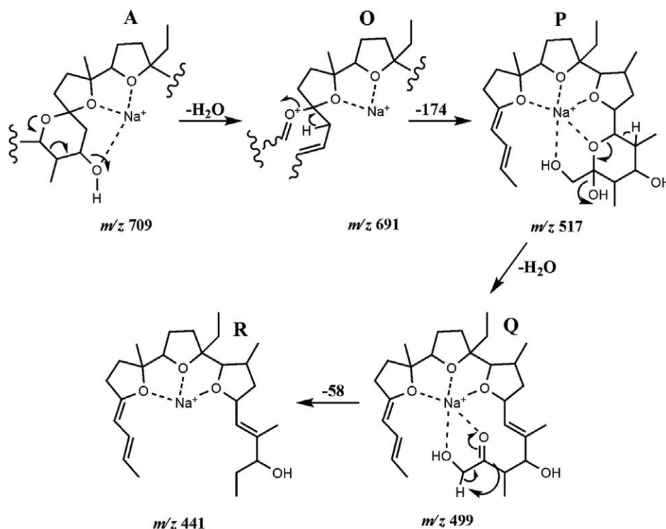
Scheme 4. Proposed mechanism of fragmentation involving the dihydropyran system and the formation of product ion m/z 441 - crucial for locating the site of hydroxylation in the MonA metabolite.
