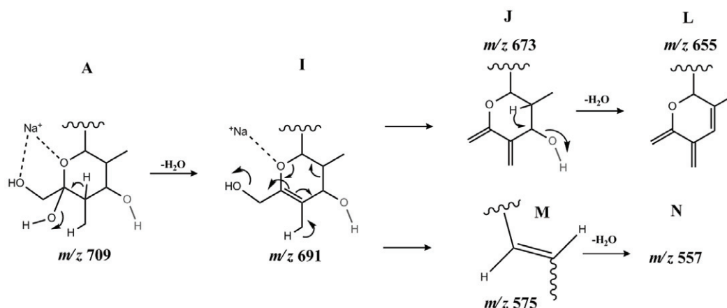
Scheme 3. The proposed fragmentation route showing the formation of product ion m/z 655.
