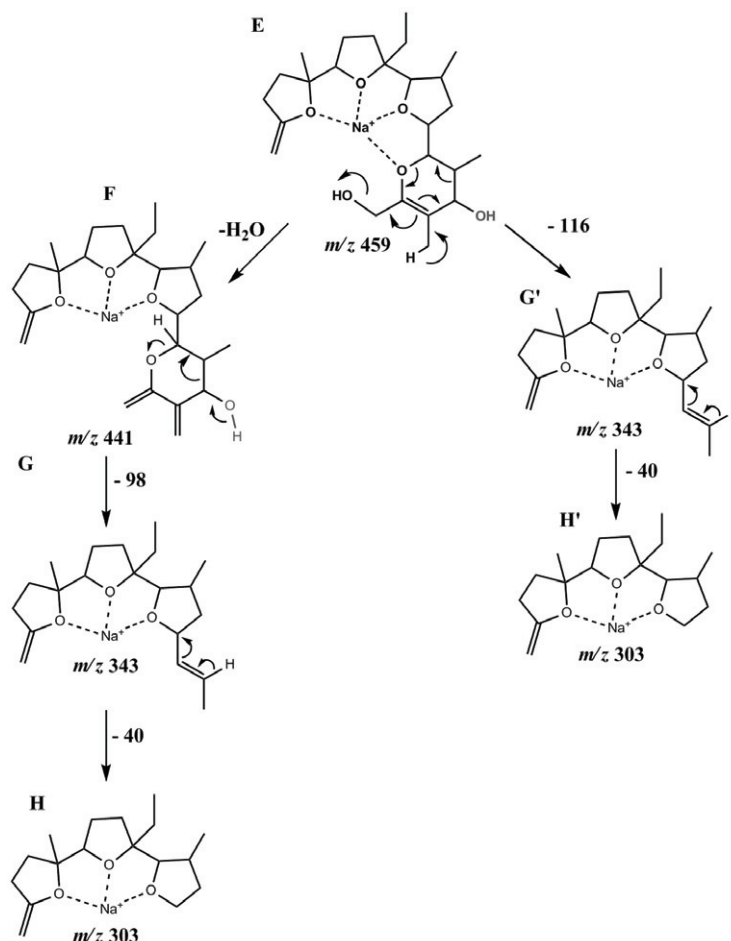
Scheme 2. The proposed fragmentation route showing the formation of product ion m/z 303 in the positive ion ESI-MS/MS of the hydroxylated metabolite of monensin A - a crucial ion for the location of the site of hydroxylation.
