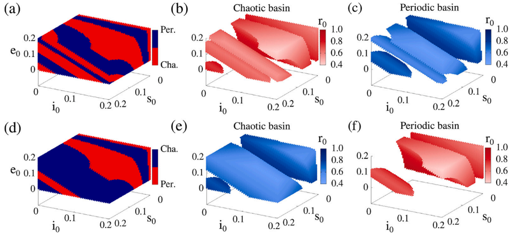
Fig. 5. Basin attraction calculated for \alpha = 100 . In panel (a) there is the total basin attraction, in panel (b) the basin of chaotic attractor, and in panel (c) the periodic basin. In panels (d), (e), and (f), we calculate the basin for \alpha = 200 . We compute the chaotic and periodic basins in the panels (e) and (f), respectively.
