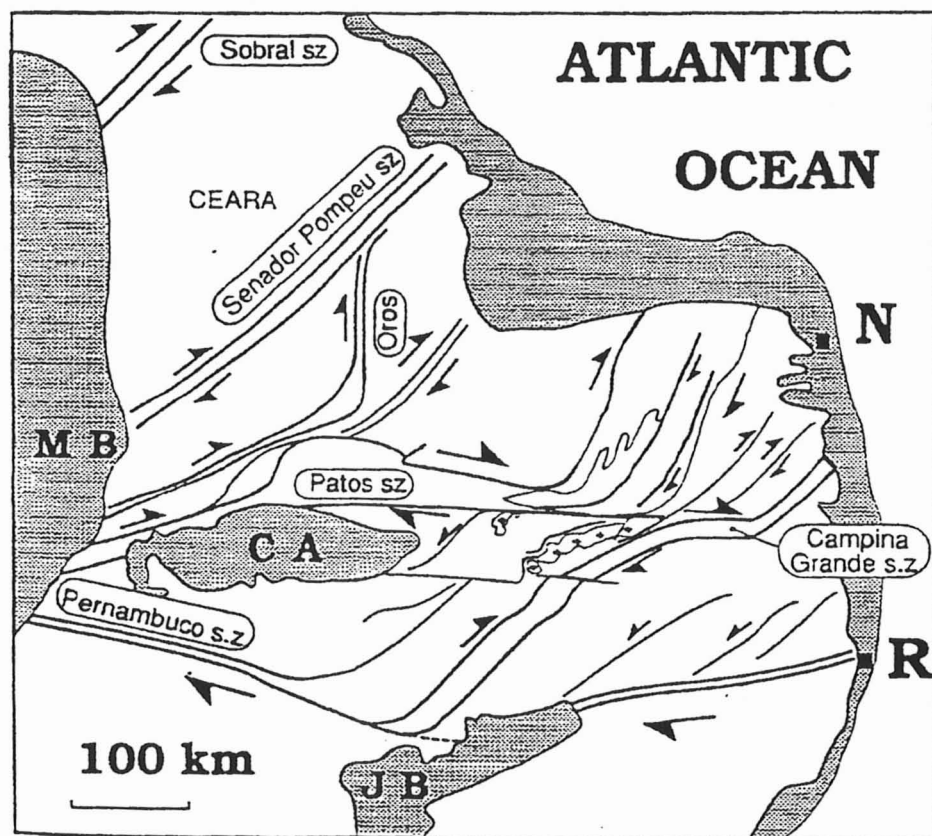
Figure 1: The continental - scale shear zone system of the Borborema Province CA= Chapada de Araripe; JB= Jotobá basin; MB= Maranhão basin; N= Natal; R= Recife
