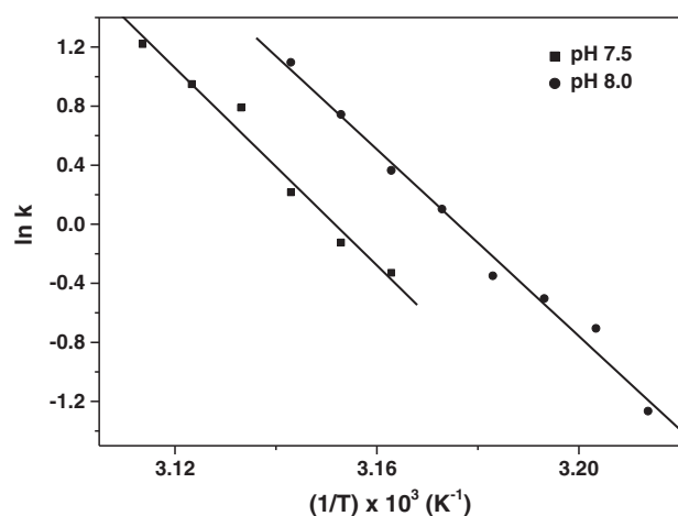
Fig. 6. Arrhenius plots for the dissociation of oxy-HbGp. The dissociation rates of oxy-HbGp were measured at 0.5 mg/mL, in acetate–phosphate–borate 30 mM, at pH 7.5 and 8.0, by DLS. The lines are the linear best fits at indicated pH values.
