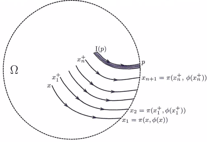
Figure 2: Given x \in \Omega , x_n \xrightarrow{n \rightarrow +\infty} p implies x_n^+ \xrightarrow{n \rightarrow +\infty} I(p) .
