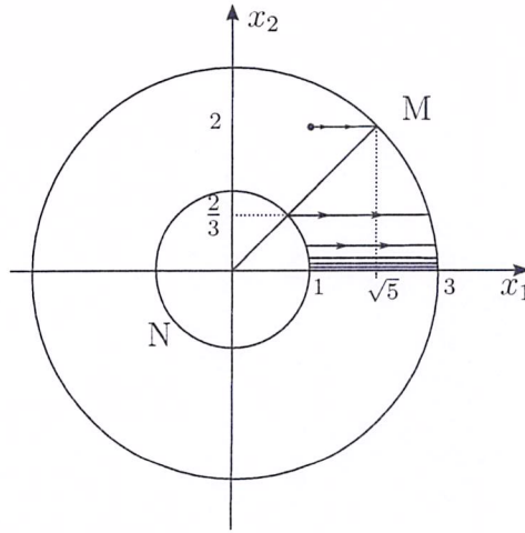
Figure 1: Trajectories of the impulsive system (1).
