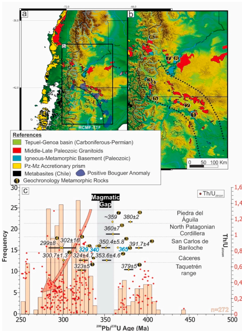
Fig. 12. a) Distribution of Paleozoic lithologies in the region based on Varella et al. (2005), Pankhurst et al. (2006), Ramos (2008) and Hervé et al. (2016). Positive Bouguer anomalies based on Renda et al. (2019). b) Location of the Central Patagonian Igneous-Metamorphic Belt c) Histogram with ^{206}\text{Pb}/^{238}\text{U} ages and Th/U ratios of individual magmatic zircons measured in the southwestern boundary of North Patagonian Massif (based on Pankhurst et al., 2006; Hervé et al., 2018 and this contribution). Metamorphic ages published by different authors: 1. This work, 2. González et al., this contribution, 3. Martínez et al. (2012), 4. Oriolo et al. (2019), 5. Pankhurst et al. (2006), 6. Urraza et al. (2008), 7. Varella et al. (2005), 8. Lucassen et al. (2004).
