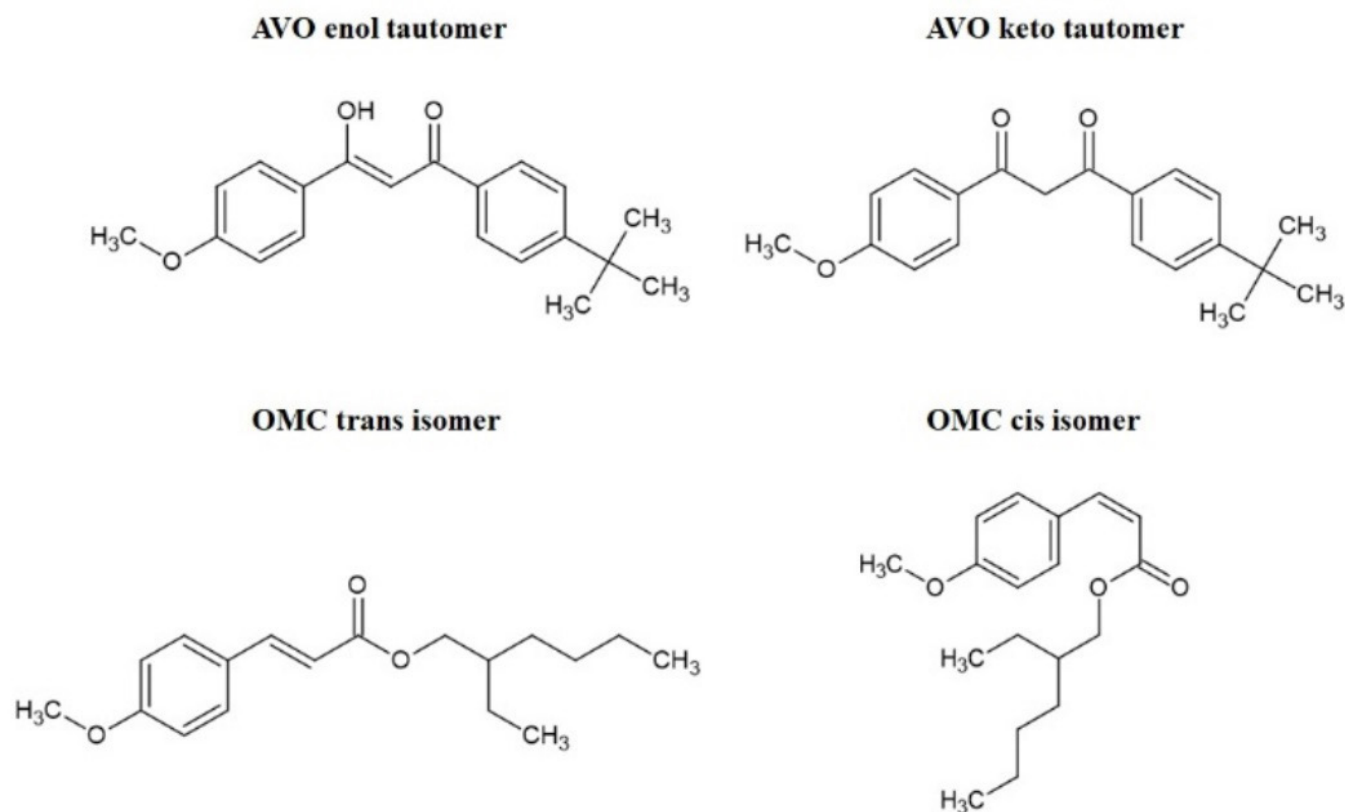
FIGURE 1 - Structural formulas of Avobenzene (AVO) and Octyl p-methoxycinnamate (OMC).
