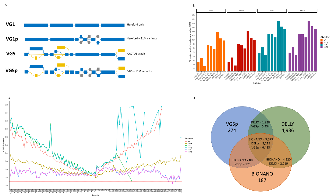
Fig. 4 Graph genome descriptions and their performances. A A cartoon representation of the four types of graph genomes considered (the linear VG1, VG1 expanded with 11M short variants (VG1p), the CACTUS VG5 graph and the CACTUS graph expanded with the 11M short variants (VG5p)). Regions indicated in blue are regions coming from the backbone sequence, those in grey are the short variants from Dutta et al. (2020), and in yellow the variants derived from the CACTUS graph; B the percent enrichment of reads mapped by vg (primary axis) using the different graphs over the bwa mem linear mapper; and C the allelic balance for the linear callers FreeBayes and GATK HaplotypeCaller compared with vg call, showing how the latter reduces the allelic bias for large variants. For other versions of this plot looking at different sets of known and novel variants see Supplementary Note 3; and D the intersection of structural variants longer than 500 bp called using the VG5p graph (blue), Delly V2 (green) and the Bionano optical mapping (orange), showing how most variants called with vg are also confirmed using one of the other methods. Note an SV called by one method may overlap more than one SV called by a different method. The source data for panels (B), (C) and (D) are provided with the paper.
