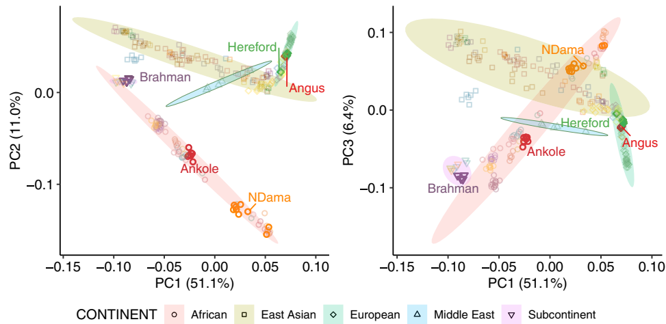
Fig. 1 Principal component analysis of the 294 cattle. The positions of the populations of origin of the five assemblies considered in this study are shown. The source data are provided with the paper.
