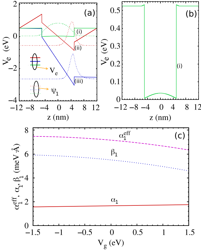
FIG. 2. (a) Self-consistent potential V_e (solid curves) and wave function profile \psi_1 of the first subband (dotted curves) for three different conditions of the built-in fields, for a GaN/ \text{Al}_{0.3}\text{Ga}_{0.7}\text{N} single well at V_g = 0 . (i) Green curves: zero built-in field (flat-band model); (ii) red curves: built-in field with periodic boundary conditions; and (iii) blue curves: built-in field with neutral surface charge boundary conditions. The energy levels (not shown) of the first subband for these three conditions are \mathcal{E}_1 = 44.9, -551.2, -2634.2 meV, respectively. (b) Blowup of the potential V_e in the flat-band model. (c) Rashba \alpha_1 , Dresselhaus \beta_1 , and effective SO \alpha_1^{\text{eff}} = \alpha_1 + \beta_1 couplings as functions of V_g . The areal electron density is kept fixed at 1.0 \times 10^{12} \text{ cm}^{-2} , so that only the first subband is occupied. The temperature is T = 2 K.
