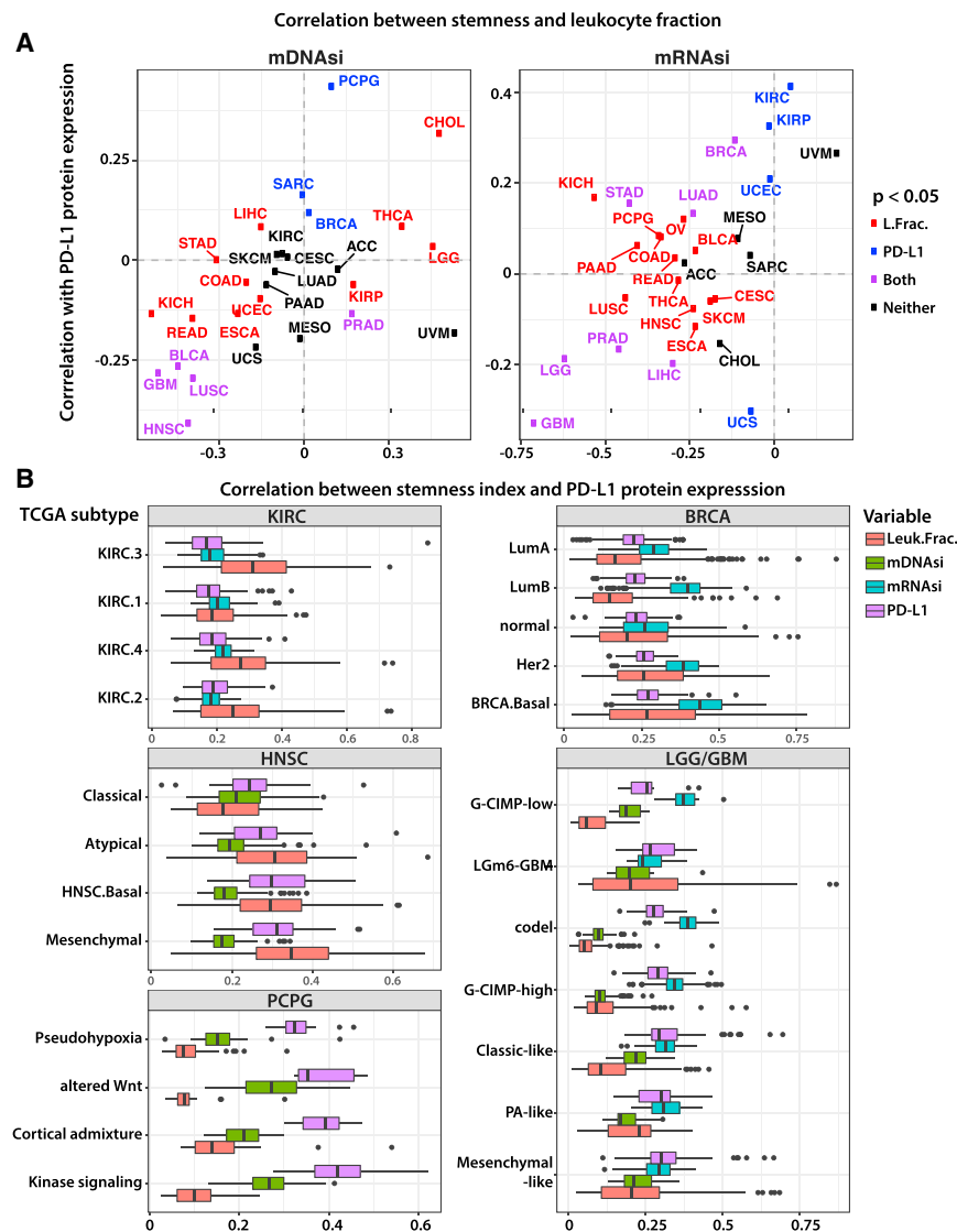
Figure 6. Association of Stemness Index with Immune Microenvironment
