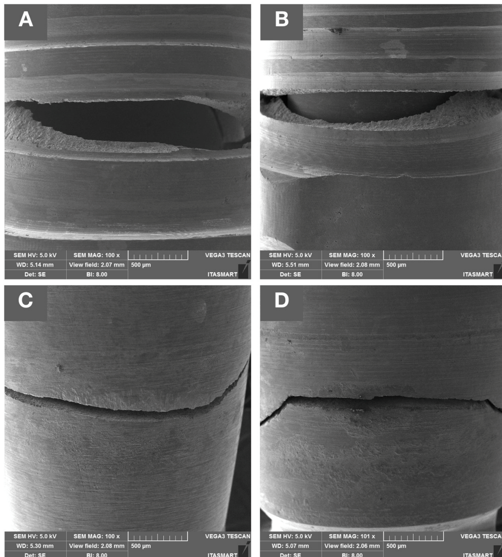
Figure 5. Scanning electron microscope images of representative samples of all experimental groups (A) Epikut 3.5, (B) GM 3.5, (C) Epikut 5, and (D) GM 5 failed during fatigue testing. While narrow implant systems presented Ti-base abutment fractures restricted to the abutment platform at the level where the crown is seated, Ti-base abutments of wide implant systems presented fractures mainly at the area of connection with the implant.
