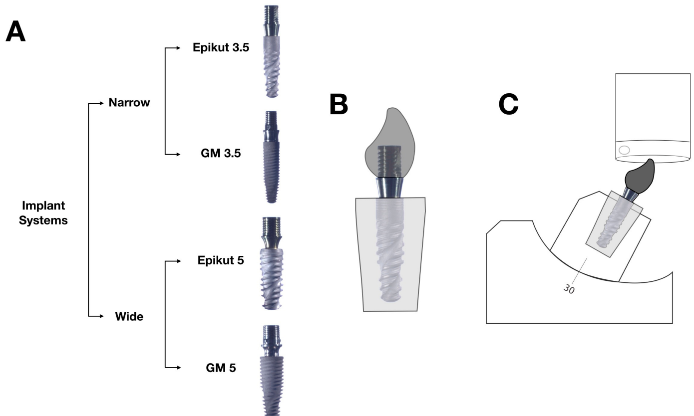
Figure 2. (A) Experimental design of the study, where two narrow (3.5 mm) and two wide (5 mm) implant systems (Epikut, SIN, National Implant System, and Grand Morse, Neodent) were tested with their respective proprietary Ti-base abutments. (B) Schematic of the implant embedded in acrylic resin up to the platform level with cobalt–chrome alloy maxillary central incisor crown cemented on the Ti-base abutment. (C) Schematic representation of experimental set-up for step stress accelerated life testing.
