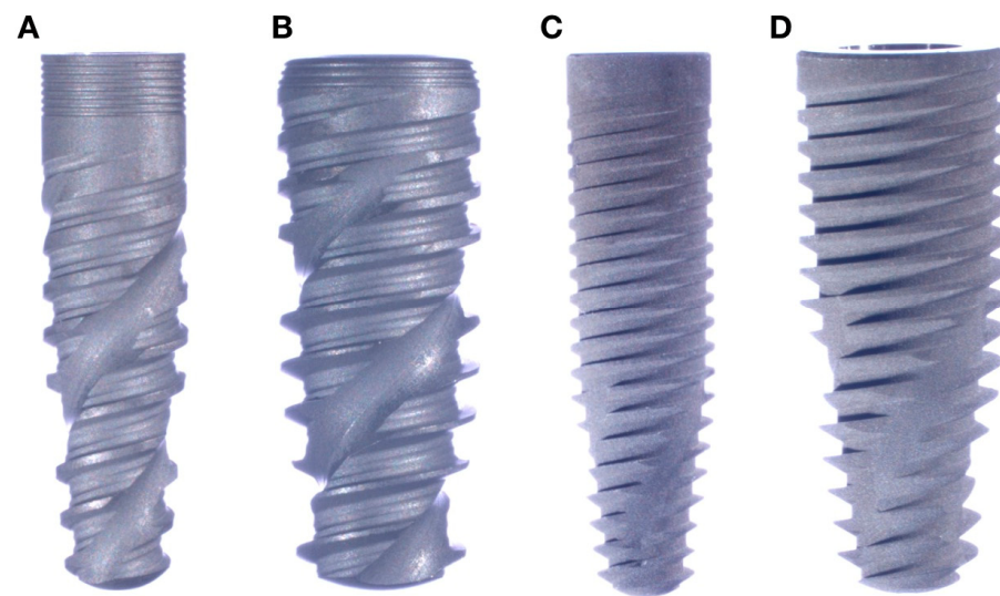
Figure 1. Macrogeometry of tested implants: Epikut 3.5 (A), Epikut 5 (B), GM 3.5 (C), and GM 5 (D).
