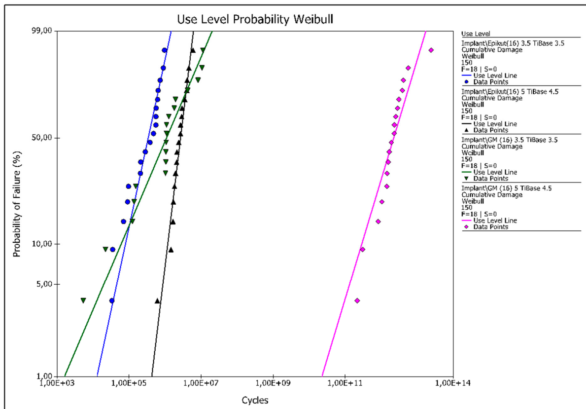
Figure 3. Use level probability Weibull curves of the experimental groups at a set load of 150 N.
