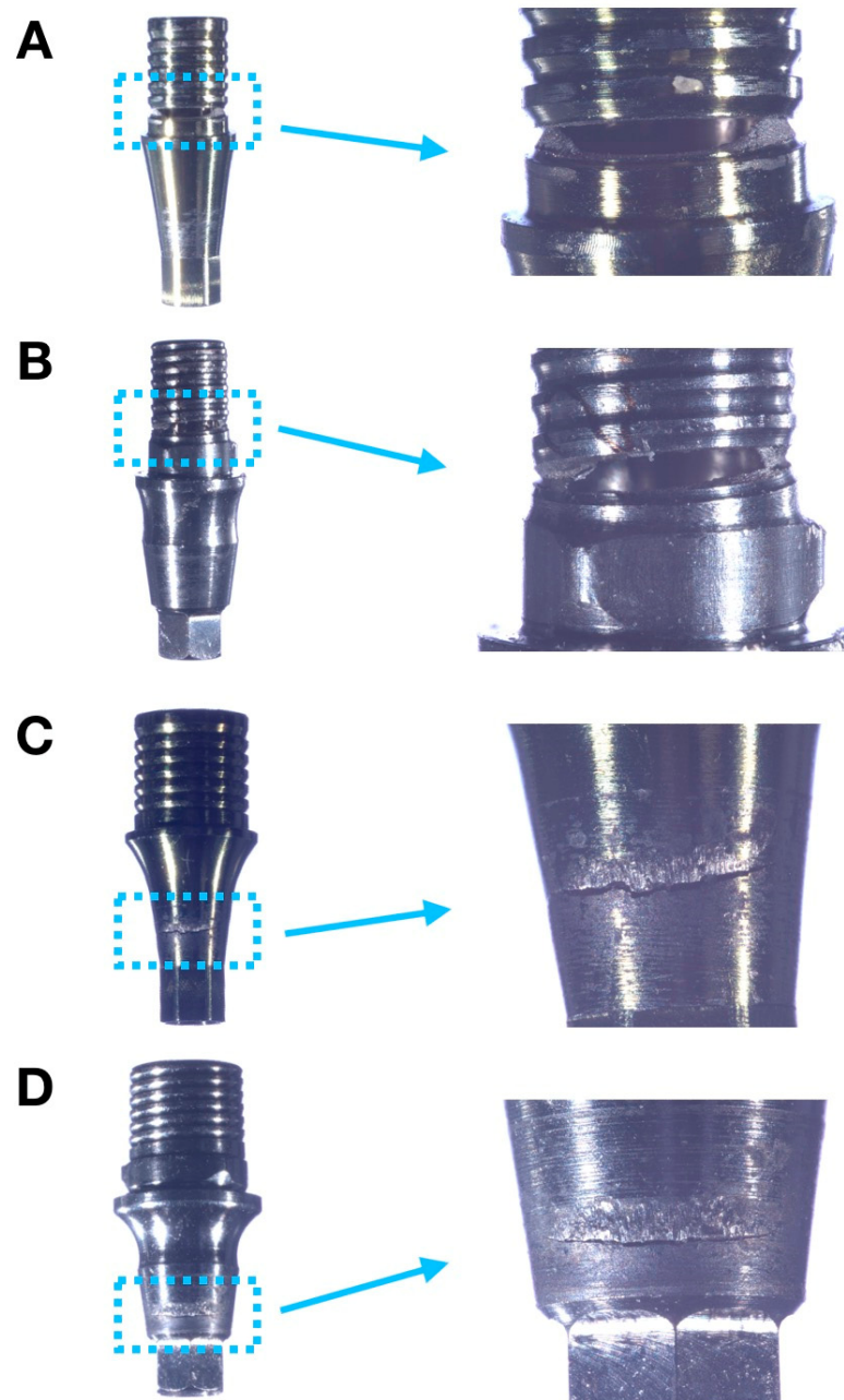
Figure 4. Failure modes of (A) Epikut 3.5, (B) GM 3.5, (C) Epikut 5, and (D) GM 5 experimental groups. Failures were comprised of Ti-base abutment fractures at the abutment platform for narrow systems (A,B) and at the area of connection with the implant for wide implant systems (C,D).
