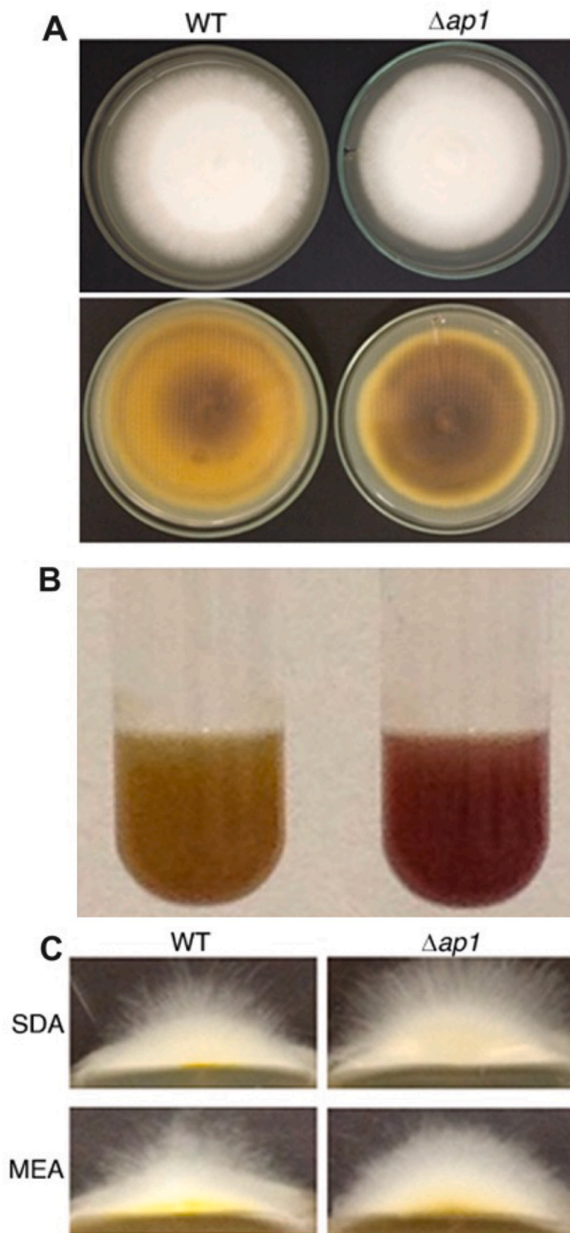
Fig. 3. ap1 gene deletion alters T. rubrum pigmentation and aerial hyphae formation. (A) Growth of wildtype (WT) and Δap1 strains in Sabouraud agar (SDA) for 21 days at 28 °C. (B) Conidial suspension of the strains after SDA growth. (C) Aerial hyphae formation in SDA and MEA, side views of the colonies were observed after 5 days at 28 °C.
