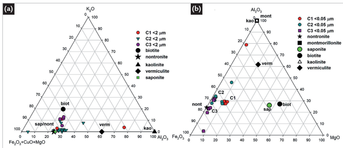
Figure 3 - Ternary diagram for clay mineral particles <2 \mu\text{m} for all samples (a). The theoretical compositions for biotite, nontronite, kaolinite and vermiculite have also been plotted. (b) - Ternary diagram of <0.05 \mu\text{m} size fraction for all samples. Their composition is close to a Fe-rich dioctahedral smectite (Petit et al. , 1992).
