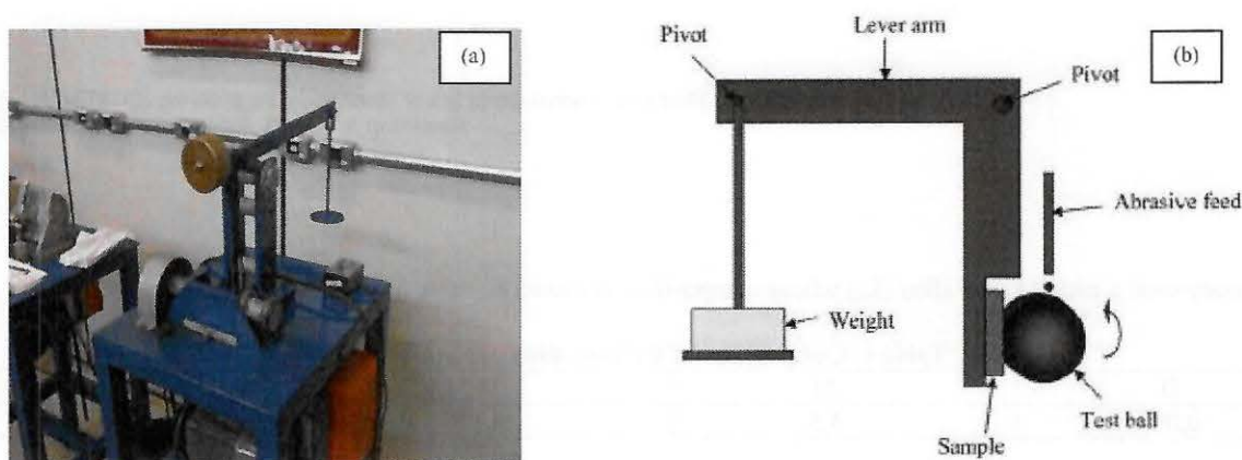
Figure 2. (a) Testing machine for micro-adhesive wear, Department of Materials Engineering - EESC-USP. (B) Illustration of the micro-adhesive wear equipment.
