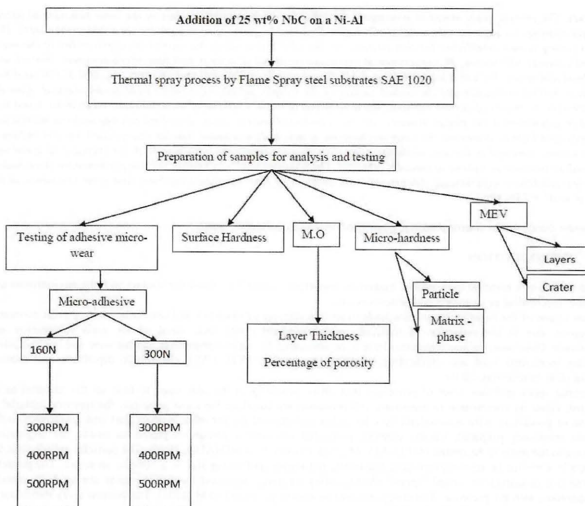
Figure 1. Flowchart of experimental work.
