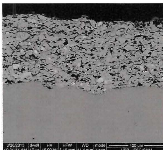
Figure 5. (a) Layer produced by the L 2 alloy.
