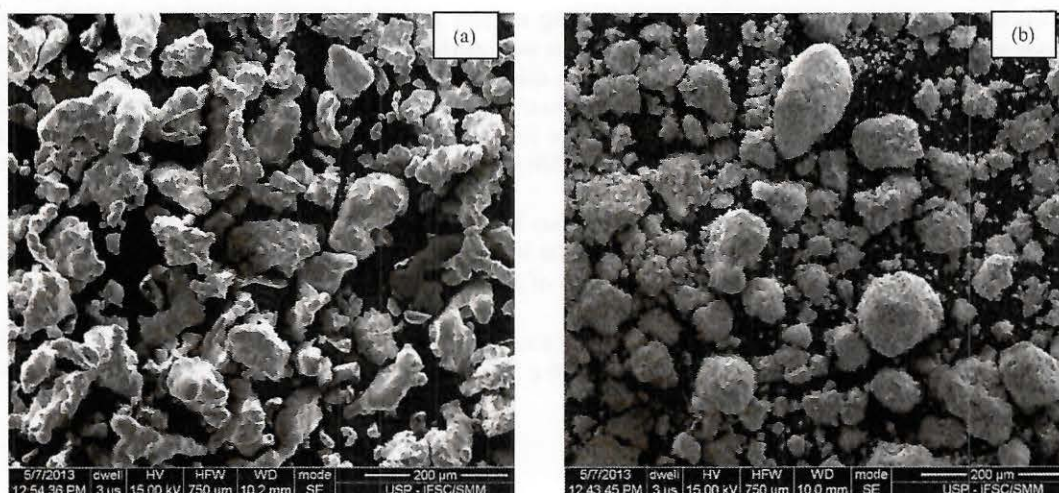
Figure 3. (A) Scanning electron micrograph of the powder alloy L 1 . (B) Scanning electron micrograph of the powder added for the production of alloy L 2 .
