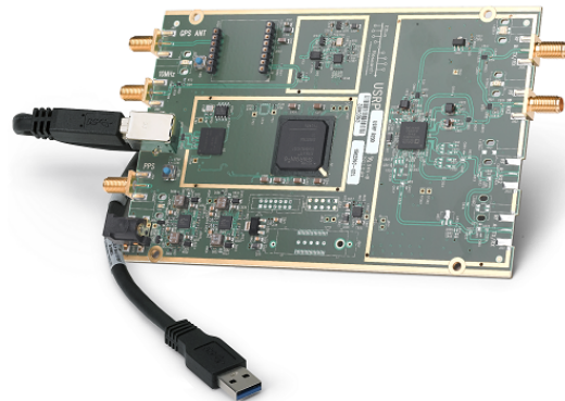
Figure 3. USRP B200 by Ettus Research. Its price is currently $905.00.
