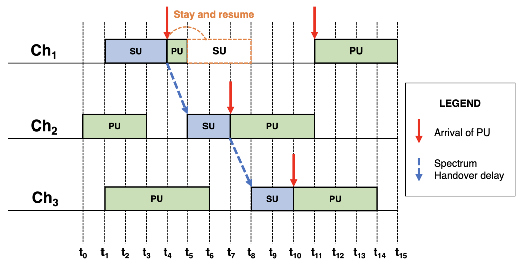
Figure 6. Spectrum handover delay caused to an SU. Adapted from the work in [87].
