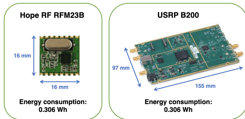
Figure 4. Physical aspects of the Hope RF RFM23B on the left and the USRP B200 on the right. The boards are shown in different size scales. Adapted from the work in [51].
