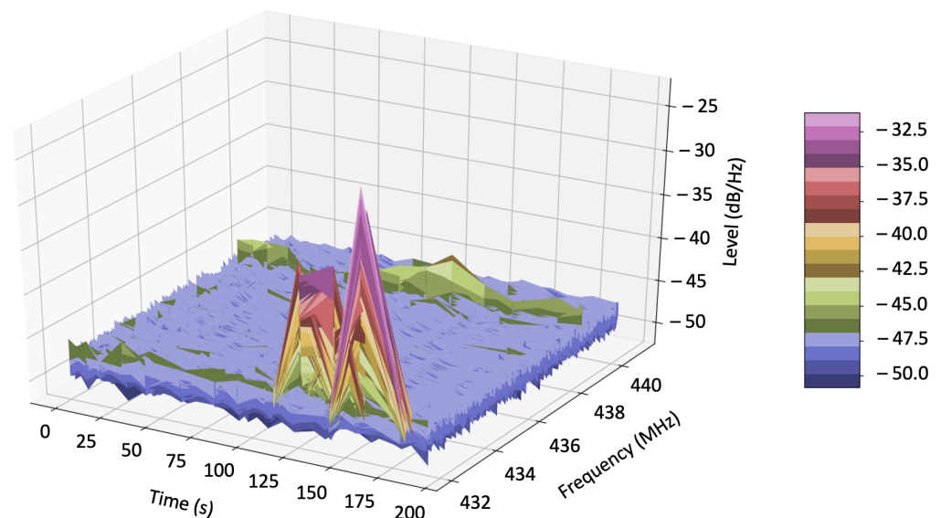
Figure 10. Data collected using the CR platform. It shows a map of the level in dB measured within the frequency range from 432 MHz to 441 MHz throughout the time.
