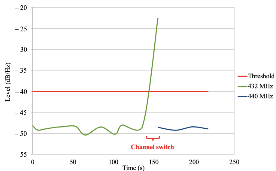
Figure 9. Data collected using the CR-based UAV. It kept using the 432 MHz frequency until it sensed a transmission level over the threshold. It then switched to its backup channel at 440 MHz.
