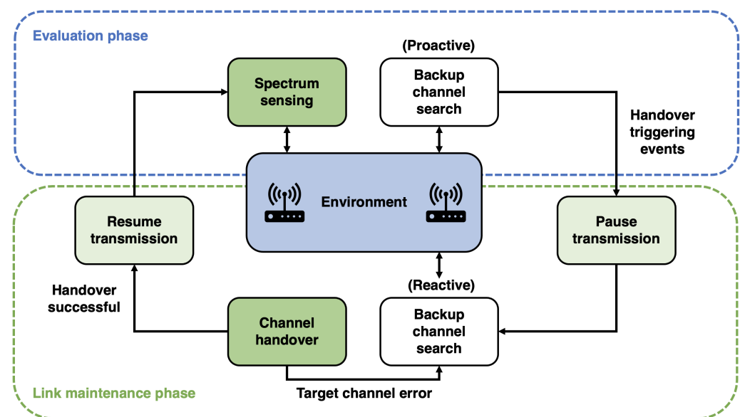
Figure 5. Spectrum handover process. Adapted from the work in [54].
