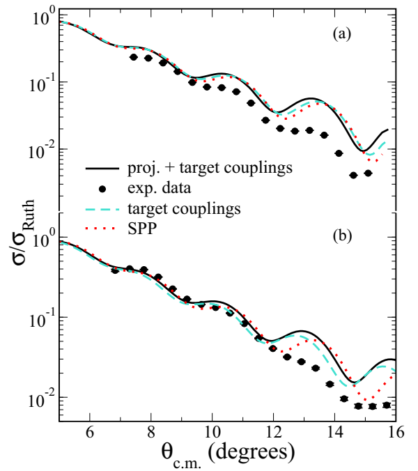
FIG. 5. Elastic angular distributions of ^{16}\text{O} + ^{27}\text{Al} (a) and ^{16}\text{O} + ^{28}\text{Si} (b) systems at 240 MeV: The dotted red line corresponds to the optical model calculation with the nuclear São Paulo potential with 1.0 and 0.78 normalization factors for the real and imaginary parts, respectively. CC calculations including inelastic states of the target only (dashed cyan line) and projectile + target excitations (black line) are also shown.
