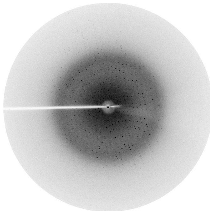
Figure 2 Typical diffraction pattern of the rx fGST crystal with a 1 ^\circ oscillation exposure. The edge of the detector corresponds to a resolution of 2.00 \text{\AA} .
