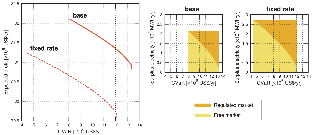
Fig. 5. Comparison between optimal portfolio solutions with either piecewise-linear ( base ) or constant ( fixed rate ) profiles of surplus electricity. Main plot (left): Pareto frontier of expected profit versus risk. Secondary plots (right): share of surplus electricity between free and regulated markets under each modeling assumption.
