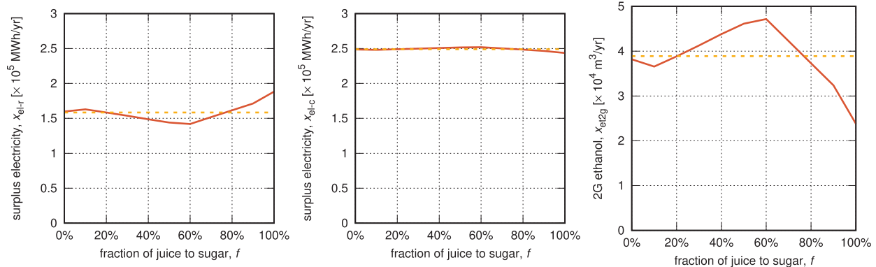
Fig. 4. Effect of the sugar-ethanol production share ( f ) on the production of: surplus electricity from the traditional Rankine cycle ( x_{el-r} , left plot); surplus electricity from the improved Rankine cycle ( x_{el-c} , middle plot); and 2G ethanol from the hydrolysis of surplus bagasse ( x_{et2g} , right plot). Solid line: simulation using the Open Sugarcane Process Simulation Platform [36]. Dashed line: average value.
