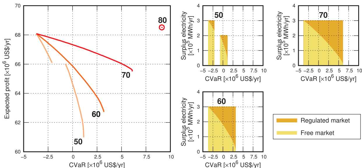
Fig. 10. Comparison between optimal portfolio solutions with electricity prices in the regulated market between US$50–80/MWh. Main plot (left): Pareto frontier of expected profit versus risk. Secondary plots (right): share of surplus electricity between free and regulated markets under each scenario.
