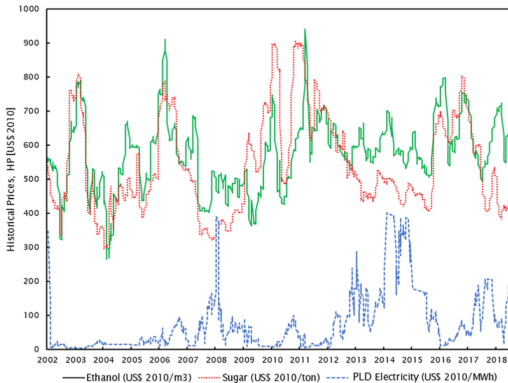
Fig. 3. Historical prices of sugar, ethanol and spot electricity (PLD).
