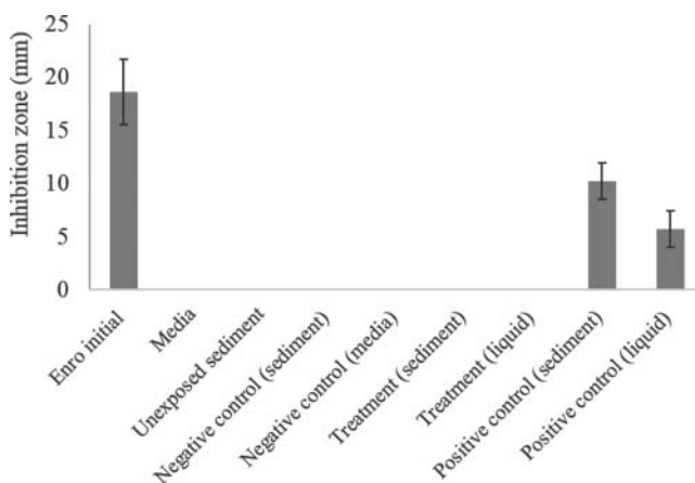
Figure 6. Antibiotic susceptibility test for enrofloxacin biodegradation in sediment from Müggelsee. Enro initial represents an enrofloxacin solution of 10 \text{ mg l}^{-1} , media was devoid of enrofloxacin (control), the negative control represented media devoid of enrofloxacin incubated in the natural sediment for 72 h, treatment represented media containing 10 \text{ mg l}^{-1} enrofloxacin incubated with the natural sediment for 72 h, and the positive control represented media containing 10 \text{ mg l}^{-1} enrofloxacin incubated with the sterilized sediment for 72 h. Data represents the average inhibition zone (mm) \pm standard deviation ( n = 4 ).
