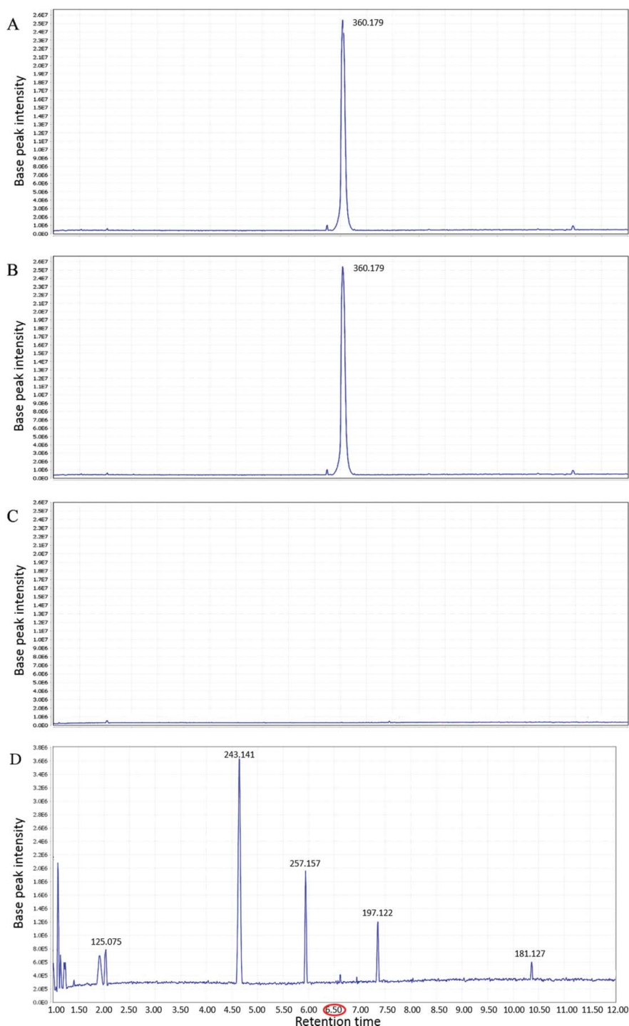
Figure 2. Total ion chromatograms of enrofloxacin (RT 6.5 min; 360 m/z ) in the control experiments via LC-ToF (ESI (+) MS- full scan mode) analyses; (A) the enrofloxacin solution (10 \text{mg l}^{-1} ) at the start of the experiment, (B) the enrofloxacin concentration after 72 h of incubation in the absence of sediment, (C) 10 ml water lacking enrofloxacin in sediment after 72 h, (D) autoclaved sediments exposed to 10 \text{mg l}^{-1} enrofloxacin for 72 h.
