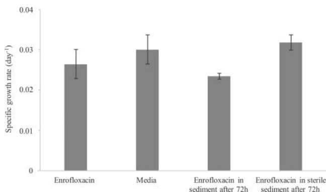
Figure 5. Specific growth rate of Desmodesmus subspicatus after 72 h of exposure to enrofloxacin at a concentration of 10 \text{ mg l}^{-1} (positive control), media devoid of enrofloxacin (negative control), the TPs of enrofloxacin after biodegradation in Müggelsee sediment after 72 h, and the products of enrofloxacin in sterilized sediment after 72 h. Data represent average \mu \pm standard deviation ( n = 4 ).
