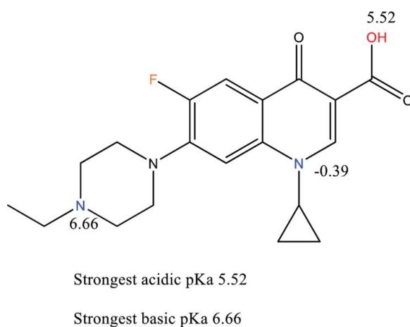
Figure 1. Chemical structure of enrofloxacin; 1-cyclopropyl-7-(4-ethylpiperazin-1-yl)-6-fluoro-4-oxo-1,4-dihydroquinoline-3-carboxylic acid.
