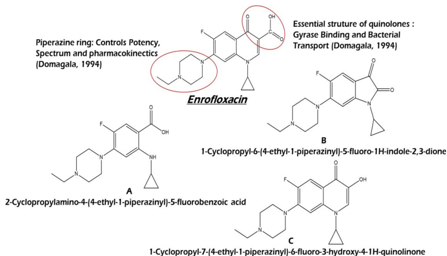
Figure 4. The three TPs of enrofloxacin identified in sediment from Müggelsee after 72 h; namely 2-Cyclopropylamino-4-(4-ethyl-1-piperazinyl)-5-fluorobenzoic acid (m/z 308), 1-Cyclopropyl-6-(4-ethyl-1-piperazinyl)-5-fluoro-1H-indole-2,3-dione (m/z 318), and 1-Cyclopropyl-7-(4-ethyl-1-piperazinyl)-6-fluoro-3-hydroxy-4-1H-quinolinone (m/z 332).
