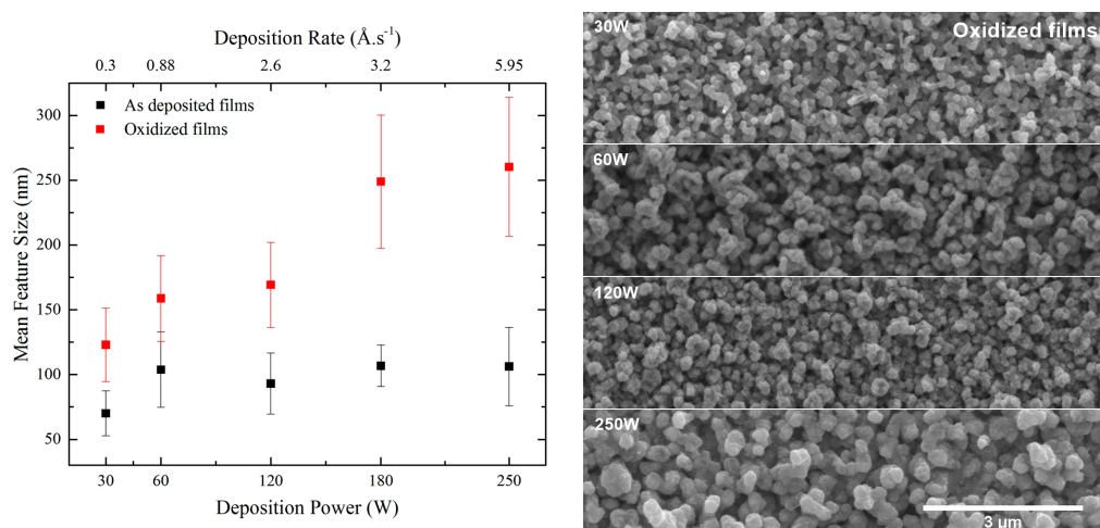
Figure 1. Mean feature size in function of power and rate deposition for metallic and oxidized films (left). Top view SEM images of films synthesized with different deposition powers (right).
