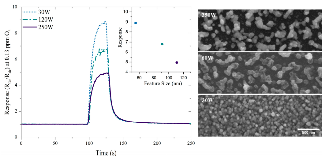
Figure 2. ZnO sputtered films sensing response at 300 °C and gas response in function of the grain size (left). SEM images for ZnO films in sensor electrodes (right).
