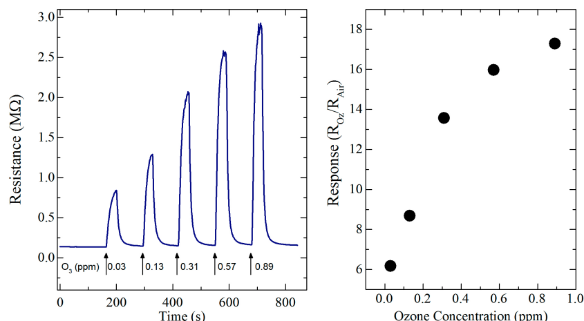
Figure 3. Change in resistance of the ZnO material deposited with 30 W and exposed at different O 3 concentrations during 30 s ( left ). Response of the sensor in function of ozone concentration ( right ).
