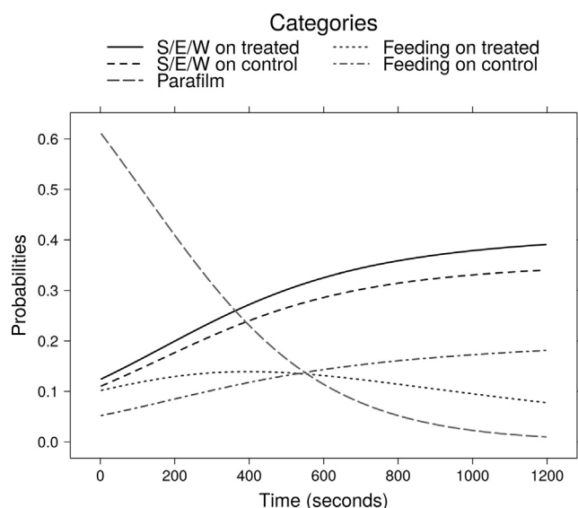
Fig. 4. Probabilities of predatory mites exhibiting each different behavior over time, as predicted by the multinomial model. The grouped category S/E/W on treated plants means the time spent by P. persimilis searching for prey (S), encountering prey (E) or walking outside leaf (W) on fungal inoculated plants (the three fungal treatments combined); and the grouped category S/E/W on control plants means the time spent by P. persimilis searching for prey (S), encountering prey (E) or walking outside leaf (W) in control non-inoculated plants; the category parafilm means the time spent by P. persimilis in the bridge of parafilm.
