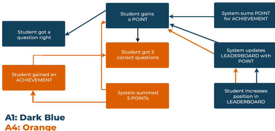
Figure 4. Interaction diagram to exemplify the decision table test
