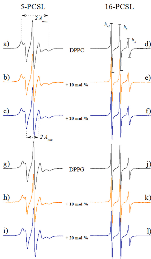
Fig. 6. Typical ESR spectra of 5-PCSL (left column) and 16-PCSL (right column) embedded into fluid vesicles of DPPC (a to f) and DPPG (g to l), in the absence and presence of 10 and 20 mol% LVX. The spectra were acquired at 50 °C, corresponding to the fluid phase of the lipids, and their total width is 100 G. The maximum and minimum hyperfine splitting ( 2A_{\max} and 2A_{\min} , respectively), and the amplitudes of the low ( h_{-1} ), central ( h_0 ) and high ( h_{+1} ) fields are indicated.
