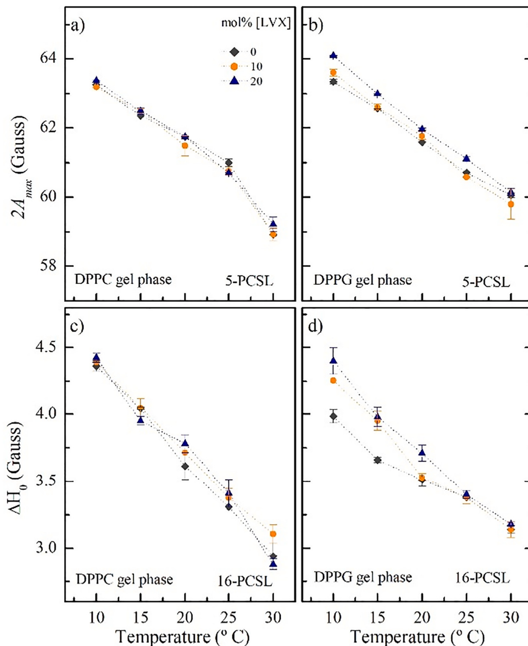
Fig. 5. Temperature dependence of the outer hyperfine splitting ( 2A_{\max} ) measured on the ESR spectrum of 5-PCSL embedded into 3 mmol L -1 gel liposomes of DPPC (a) and DPPG (b). Temperature dependence of the central field line width ( \Delta H_0 ) measured on the ESR spectrum of 16-PCSL embedded into 3 mmol L -1 gel liposomes of DPPC (c) and DPPG (d). The data were obtained in the absence of LVX (dark gray diamond), in the presence of 10 mol% LVX (orange circle), and 20 mol% LVX (blue triangle). Error bar indicates standard deviation of at least three experiments with different samples. If not shown, the deviation was found to be smaller than the symbol.
