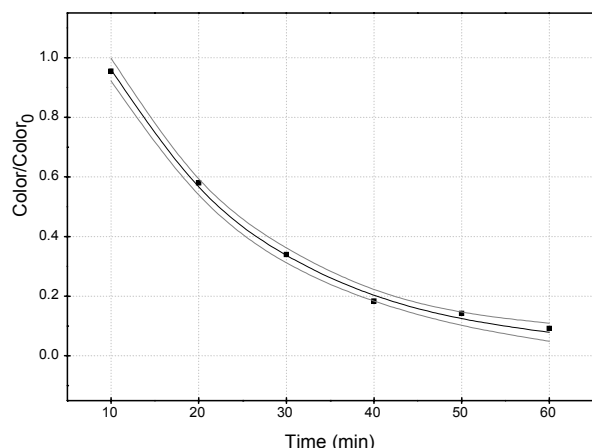
Figure 4: Color removal kinetics (photocatalysis) with the 95% confidence interval (gray). Conditions: pH 7.0, T = 25 °C, 2.0 g TiO 2 L -1 ; kinetic parameters: k = (5.4 \pm 0.92) \times 10^{-2} \text{ min}^{-1} , R^2 = 0.991 .
