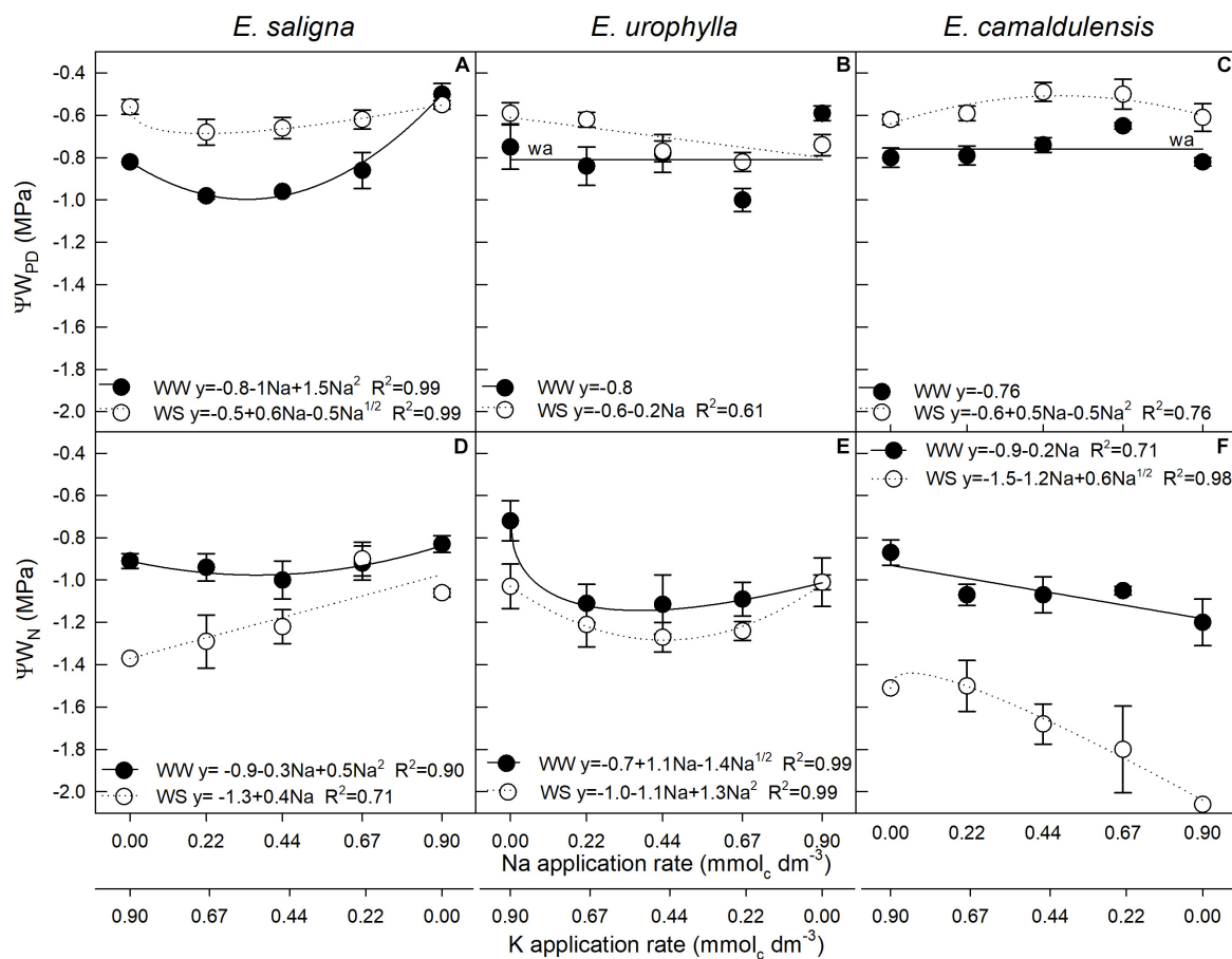
FIGURE 4 | Predawn ( \Psi_{wPD} ) (A-C) and noon ( \Psi_{wN} ) (D-F) leaf water potentials of Eucalyptus saligna (A,D), Eucalyptus urophylla (B,E), and Eucalyptus camaldulensis (C,F) seedlings under K partial replacement by Na in well-watered (WW) and water-stressed (WS) conditions. Vertical bars indicate standard errors between blocks ( n = 4 ).
