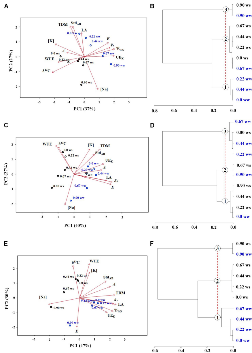
FIGURE 6 | Principal component analysis (PCA) (A,C,E) and hierarchical cluster analyses (B,D,F) of Eucalyptus saligna (A,B), Eucalyptus urophylla (C,D), and Eucalyptus camaldulensis (E,F) seedlings under K partial replacement by Na (0, 0.22, 0.44, 0.67, and 0.90 mmol c dm -3 of Na) in well-watered (WW) and water-stressed (WS) conditions.
