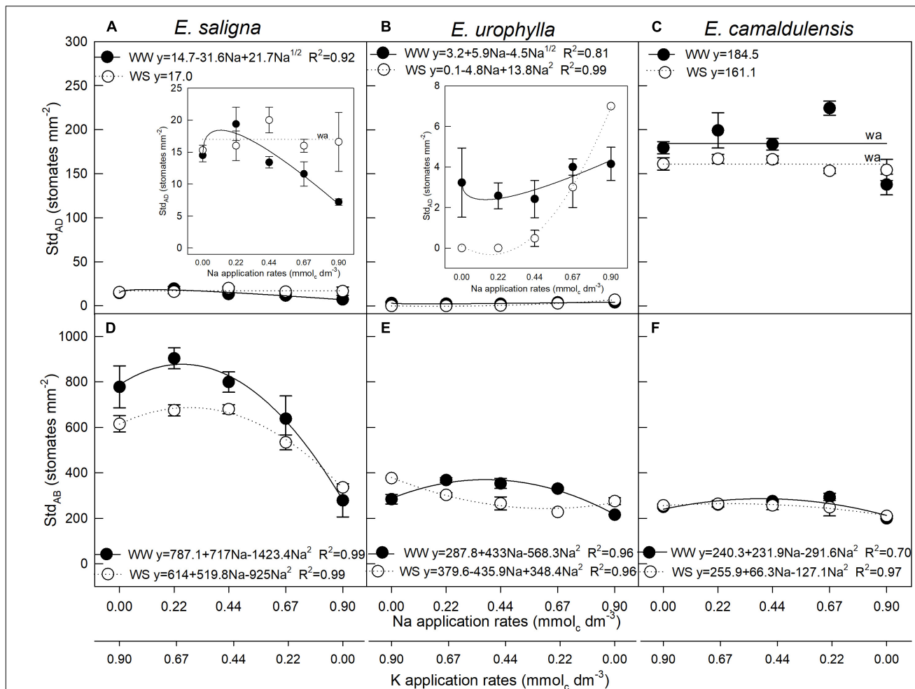
FIGURE 1 | Stomatal density of the adaxial (Std AD ) (A–C) and abaxial (Std AB ) (D–F) leaf surfaces of Eucalyptus saligna (A,D), Eucalyptus urophylla (B,E), and Eucalyptus camaldulensis (C,F) seedlings under K partial replacement by Na in well-watered (WW) and water-stressed (WS) conditions. Vertical bars indicate standard errors among blocks ( n = 4 ). The adjustment model is indicated by not significant (ns) and without suitable adjustment (wa).
