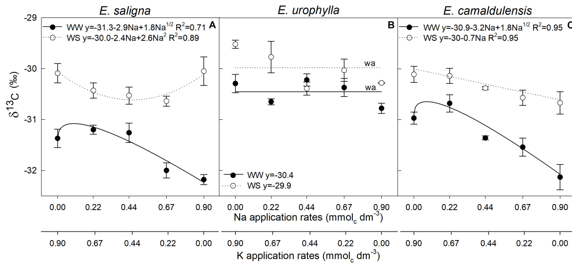
FIGURE 3 | Leaf Carbon Isotope Composition ( \delta^{13}\text{C}\text{‰} ) of Eucalyptus saligna (A), Eucalyptus urophylla (B), and Eucalyptus camaldulensis (C) seedlings under K partial replacement by Na in well-watered (WW) and water-stressed (WS) conditions. Vertical bars indicate standard errors among blocks ( n = 4 ). The adjustment model is indicated by not significant (ns) and without suitable adjustment (wa).
