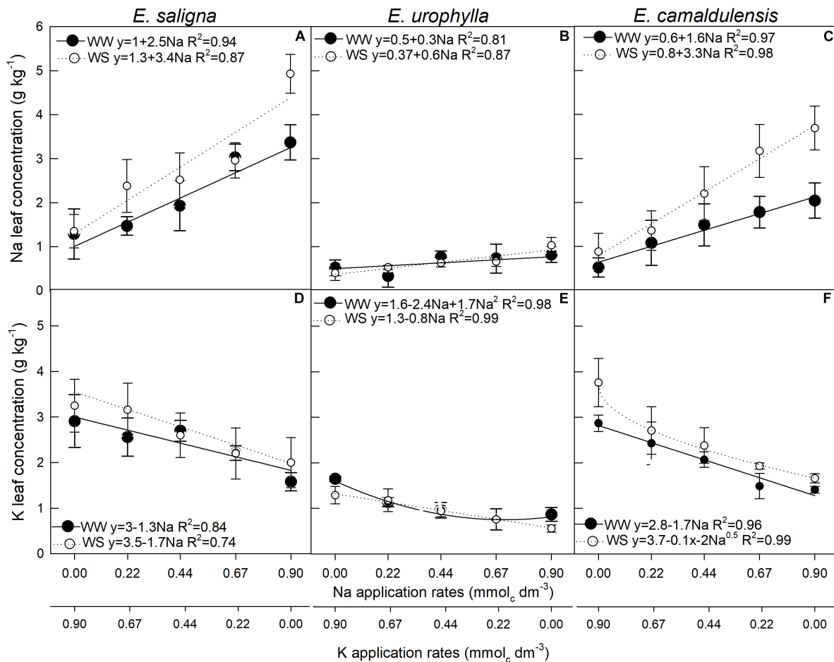
FIGURE 5 | Leaf Na (A–C) and leaf K (D–F) concentrations of Eucalyptus saligna (A,D), Eucalyptus urophylla (B,E), and Eucalyptus camaldulensis (C,F) seedlings under K partial replacement by Na in well-watered (WW) and water-stressed (WS) conditions. Vertical bars indicate standard errors between blocks ( n = 4 ).
