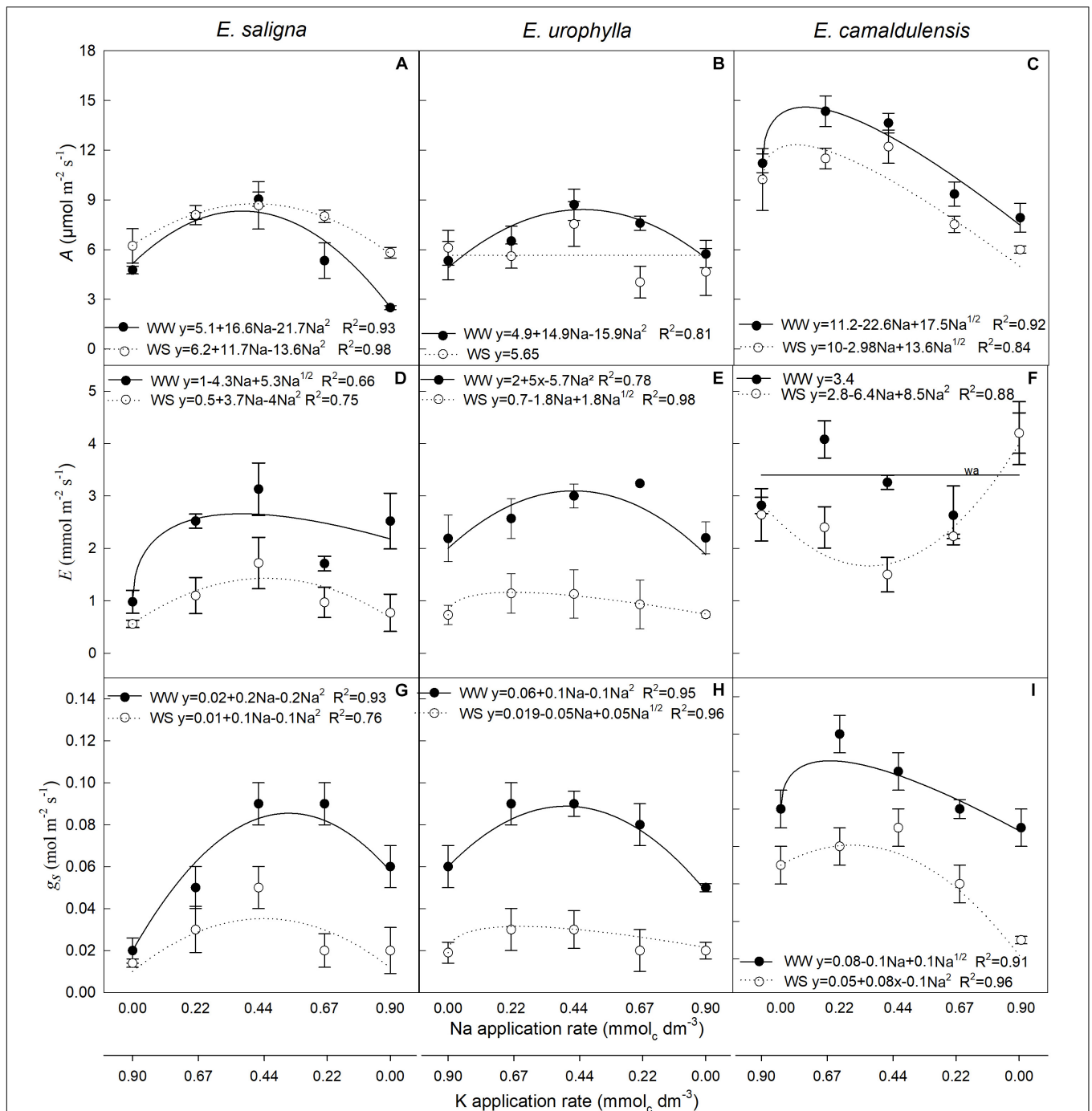
FIGURE 2 | Photosynthetic rate (A) (A–C), leaf transpiration rate (E) (D–F), and stomatal conductance ( g_s ) (G–I) in the leaves of Eucalyptus saligna (A,D,G), Eucalyptus urophylla (B,E,H), and Eucalyptus camaldulensis (C,F,I) seedlings under K partial replacement by Na in well-watered (WW) and water-stressed (WS) conditions. Vertical bars indicate standard errors between blocks ( n = 4 ). The without suitable adjustment of a model is indicated by wa.
