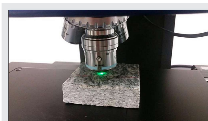
Figure 4. Interferometer in active measuring, also showing object holder.
