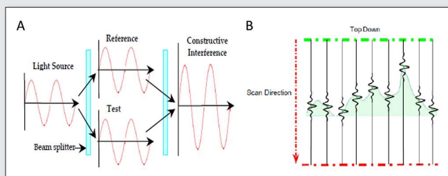
Figure 2 3 . (A) Superposition principle on an interferometer showing the combination of reference and test beams, resulting in constructive interference 4 . (B) Interferometer scanning process, which finds the surface height by analysing the fringe patterns.
