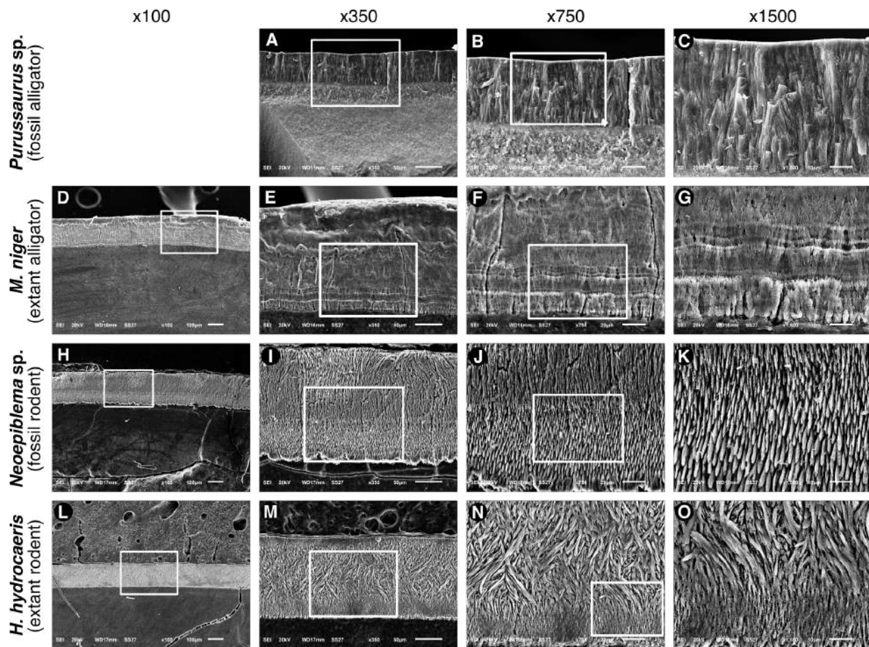
Figure 5. Images obtained by SEM analysis of enamel cross-sections from the four (4) specimens Purussaurus sp., Melanosuchus niger , Neopiblema sp., and Hydrochoerus hydrochaeris . (A–C), the enamel of Purussaurus sp. is formed by rod-like structures that run roughly perpendicular to the enamel surface and dentine–enamel junction (DEJ), having a width of approximately 5 \mu\text{m} . (D–G), Melanosuchus niger has a typical aprismatic structure, showing growth lines that are likely to be the equivalent to the mammalian Retzius lines. These lines were localized near the DEJ and are likely to represent periods of physiological stress during enamel synthesis. (H–K), the enamel of Neopiblema sp. is formed by prisms that are roughly parallel and perpendicular to the DEJ and enamel surface. The DEJ exhibits an irregular surface. (L–O), the enamel of Hydrochoerus hydrochaeris shows 2 distinct patterns of prisms arrangement. The prisms run nearly parallel from the DEJ and extend approximately 25–30 \mu\text{m} near the DEJ. A thin layer of parallel prisms is also observed near the enamel surface. In most parts of enamel, the prisms exhibit a pattern of intense decussation.
