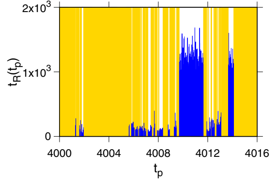
FIG. 6. Time for the synchronized state be restored, t_R , as function of the perturbation instants, t_p . The perturbation is given by \Delta_{19} = (0.0, 0.97, -1.14) . The yellow (light-gray) bars delimitate perturbation instants for which the system desynchronizes, while the height of the blue (dark-gray) bars represents the restoring time of synchronization.
