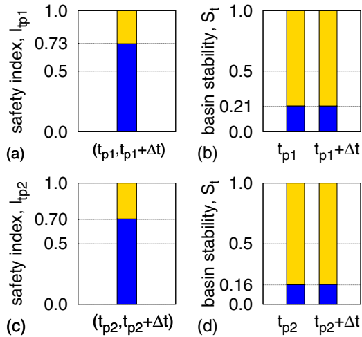
FIG. 4. In (a) the blue (dark-gray) color indicates the safety index between synchronization diagrams obtained for two consecutive states \mathbf{v}_S(t_{p1}) at t_{p1} = 4005.97 and \mathbf{v}_S(t_{p1} + \Delta t) with \Delta t = 10^{-2} . (b) The blue (dark-gray) color indicates the corresponding basin stability of the synchronization diagrams analyzed in (a). In (c), the blue (dark-gray) color indicates the safety index for two different consecutive states \mathbf{v}_S(t_{p2}) at t_{p2} = 4009.95 and \mathbf{v}_S(t_{p2} + \Delta t) with \Delta t = 10^{-2} . (d) The blue color (dark gray) indicates the corresponding basin stability of the synchronization diagrams analyzed in (a).
