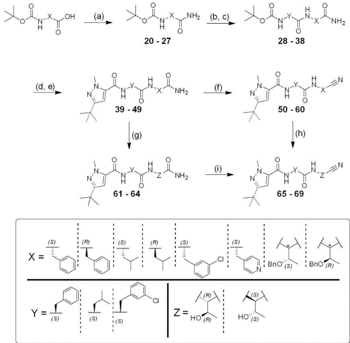
Fig 2. General synthesis of compounds 50–60, 65–69. Reagents and conditions: a) Isobutyl chloroformate, \text{NH}_4\text{Cl} 2 M, DIPEA, DMF, 0 °C to rt, 20 h; b) TFA, \text{CH}_2\text{Cl}_2 , 0 °C to rt, 2 h; c) HATU, DIPEA, Boc-AA-OH, DMF, rt, 18 h; d) TFA, \text{CH}_2\text{Cl}_2 , 0 °C to rt, 2 h; e) TBTU, DIPEA, 3-( tert -butyl)-1-methyl-1 H -pyrazole-5-carboxylic acid, DMF/ \text{CH}_2\text{Cl}_2 , rt, 18 h; f) Cyanuric chloride, DMF, 0 °C to rt, 0.5 h; g) \text{H}_2 (1 atm), Pd/C, rt, 18 h; h) DDQ, \text{CH}_2\text{Cl}_2 , rt, 3–5 days; i) TFAA, DIPEA, THF, 0 °C to rt, 2 h.
