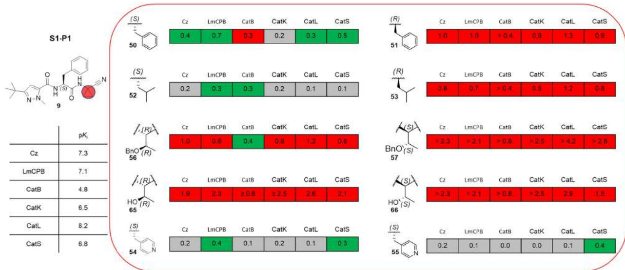
Fig 8. SAR summary for P1-S1/S1' interactions. Values are reported as differences in pK_i and are color-coded as red (negative), green (positive), grey (no significant difference, \Delta pK_i < 0.2 ).
