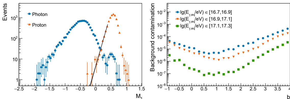
Figure 9. Left: The M_{b=1} distributions for simulated photon- and proton-initiated events for energies \lg(E_{\gamma,eq}/\text{eV}) \in (16.7, 16.9) . The uncertainty in bins with fewer than ten entries is the asymmetric confidence belt calculated with the Feldman-Cousins method at 95% confidence level [67]. The fit to the proton tail employed to estimate the background contamination is displayed as a black band. Right: The average background contamination for the quoted energy bins in terms of b for a fixed signal efficiency of 50%.
