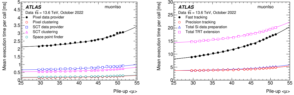
Figure 22. Execution times for the muon isolation track reconstruction shown as a function of the average pile-up. (Left) Detailed breakdowns for the Pixel and SCT data preparation components. (Right) The muon isolation tracking, the combined silicon data preparation and TRT extension times. Solid lines show ad hoc fits to data to guide the eye. Only statistical uncertainties are shown.
