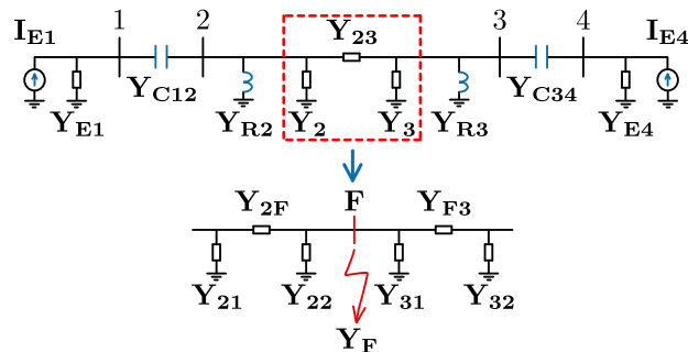
FIGURE 5. Substitution of the pre-fault line for the post-fault sections with the new fault node F in generic electric grid.
