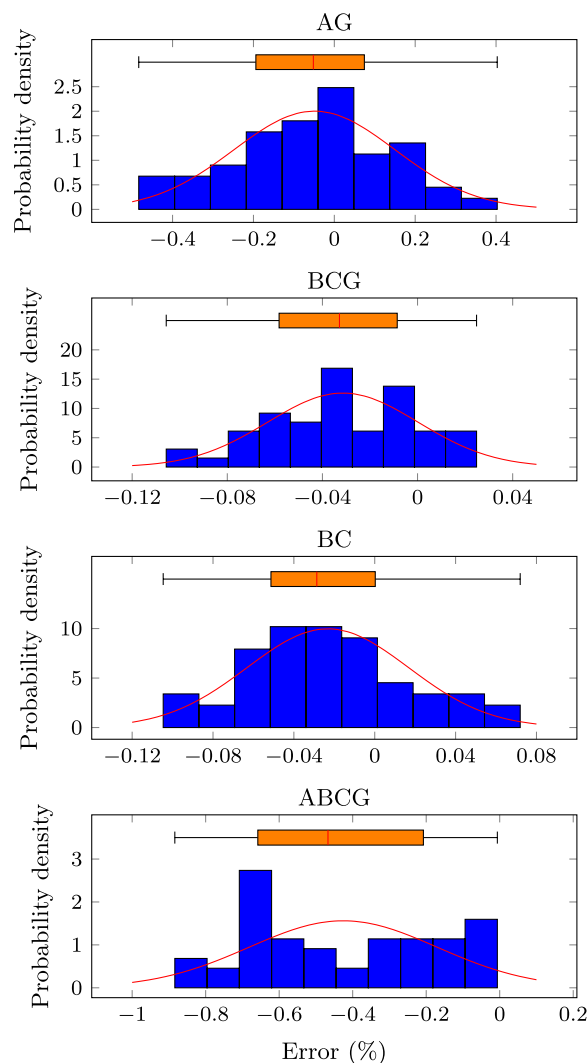
FIGURE 14. Fault distance errors considering deviations on equivalents for all fault types. Faults at 50% (128 [km]) from L terminal, resistance combination 5 (5/50), and phasors extracted from steady-state.
