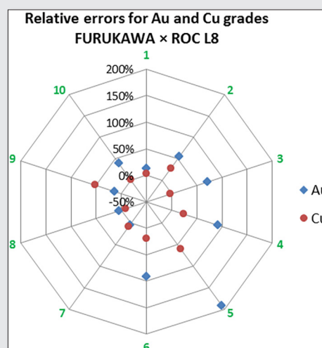
Figure 3. Furukawa relative errors for copper and gold grades compared to RC ROC L8 twin holes.
