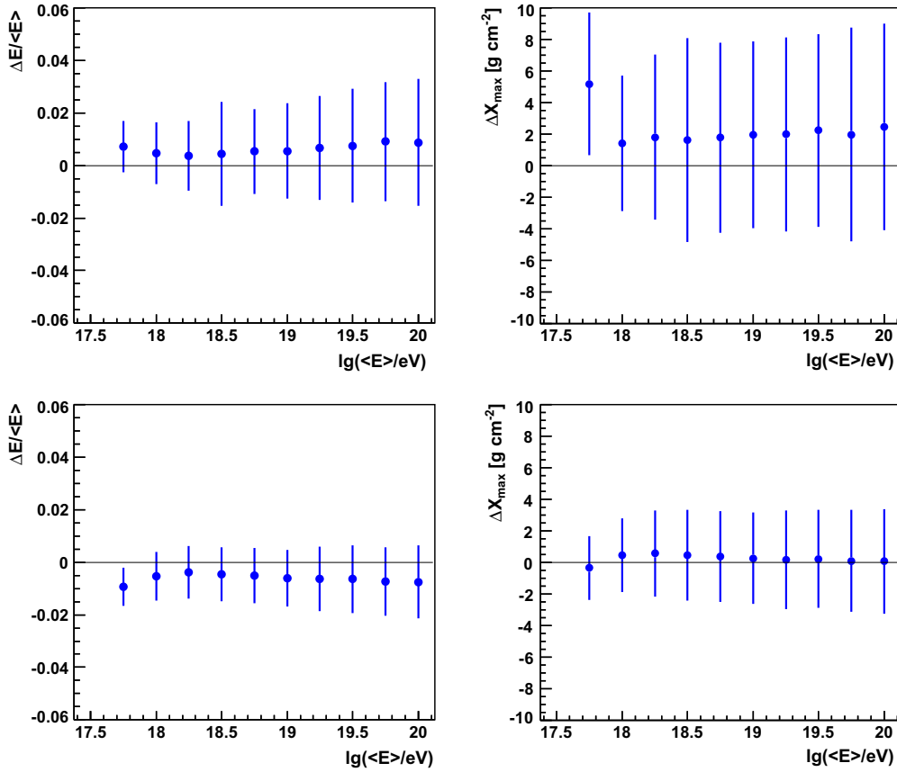
Fig. 14. Energy difference (left) and X_{\text{max}} difference (right) vs. reconstructed FD energy for simulated showers. The influences of the monthly models (top) and of GDAS data (bottom) are shown. Error bars denote the RMS spread.
