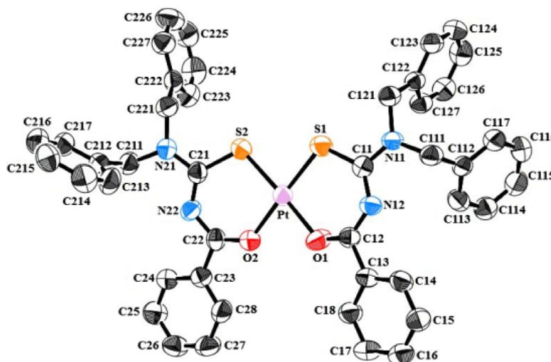
Figure 1 ORTEP view of the title compound, with atom-numbering. Hydrogen atoms are omitted for clarity. Displacement ellipsoids are drawn at the 50% probability.
