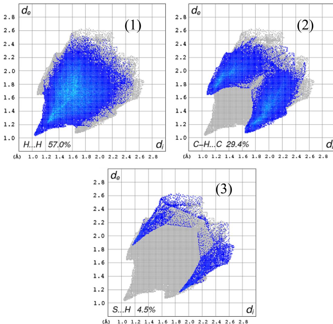
Figure 3 Fingerprints of the title compound, (a) \text{H}\cdots\text{H} , (b) \text{C}\cdots\text{H} , (c) \text{S}\cdots\text{H} . The outline of the full fingerprint is shown in gray.
