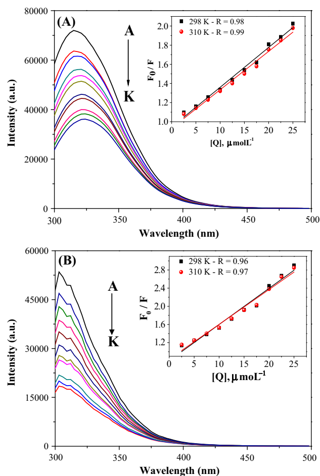
Figure 4 Fluorescence emission spectra of the BSA (2.5 \mu\text{M} ; \lambda_{\text{ex}} = 270 \text{ nm} ) and HSA (5 \mu\text{M} ; \lambda_{\text{ex}} = 270 \text{ nm} ) at different concentrations of complex Pt(II) at 310 K.
