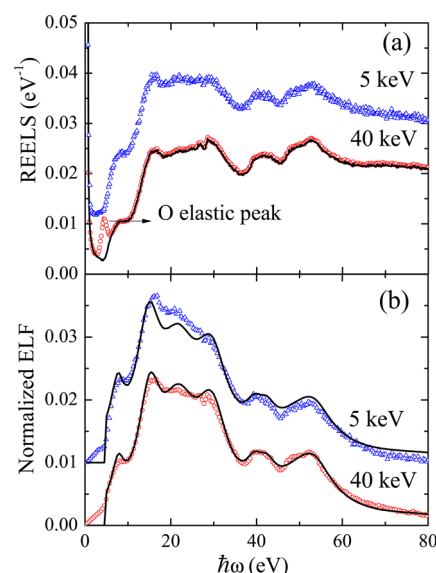
Figure 1. (a) Measured REELS energy spectrum (symbols) in \text{Ta}_2\text{O}_5 films for incident electron energies of 5 and 40 keV. A separate O elastic peak can be seen for electrons at 40 keV, and after removing it we obtain the black line. (b) Normalized optical energy loss function of \text{Ta}_2\text{O}_5 (symbols) for both incident electron energies, and the corresponding fits obtained using the QUEELS package 28 (solid lines). For clarity, the data corresponding to 5 keV electrons are offset by 0.01 in both panels.
