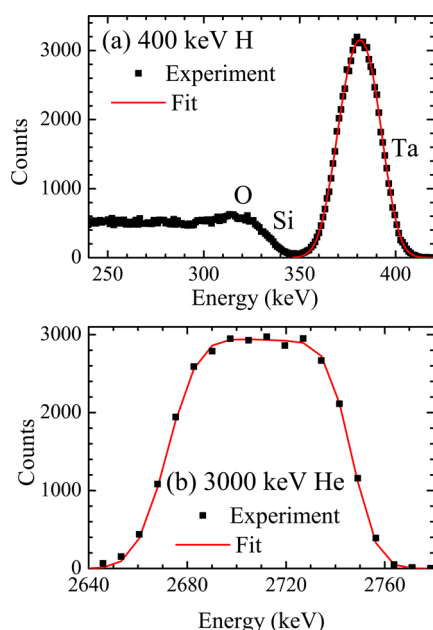
Figure 4. (a) RBS spectrum (symbols) used to extract the \text{Ta}_2\text{O}_5 stopping cross section: a 74.5 nm \text{Ta}_2\text{O}_5 film bombarded by a 400 keV H beam at normal incidence. It is possible to see the O signal from the film, as well as the Si structure from the substrate. (b) RBS spectrum used to extract the energy-loss straggling of \text{Ta}_2\text{O}_5 : a 94.5 nm \text{Ta}_2\text{O}_5 film was bombarded by a 3000 keV He beam at the incidence angle of \theta_i = 45^\circ . In both cases, symbols correspond to present RBS measurements, whereas the solid lines represent the fit to the Ta signal.
