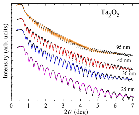
Figure 3. Measured X-ray reflectivity spectra (symbols) and corresponding WinGIXA simulated spectra (solid curves) for four Si(100)/ \text{Ta}_2\text{O}_5 films, labeled with the corresponding thickness of the \text{Ta}_2\text{O}_5 films.
