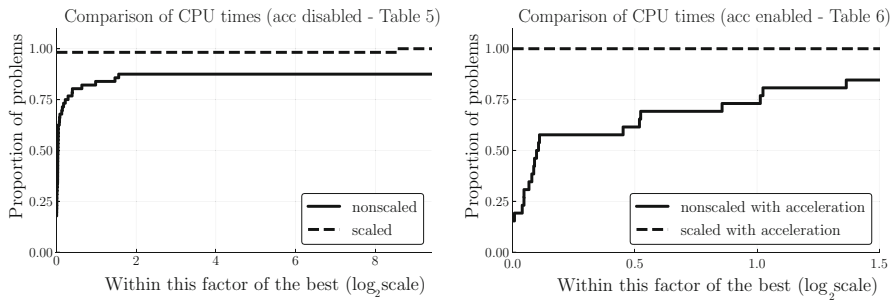
Fig. 1 Visual representation of the data of Tables 5 and 6, emphasizing the problems where the nonscaled and scaled variants performed differently
