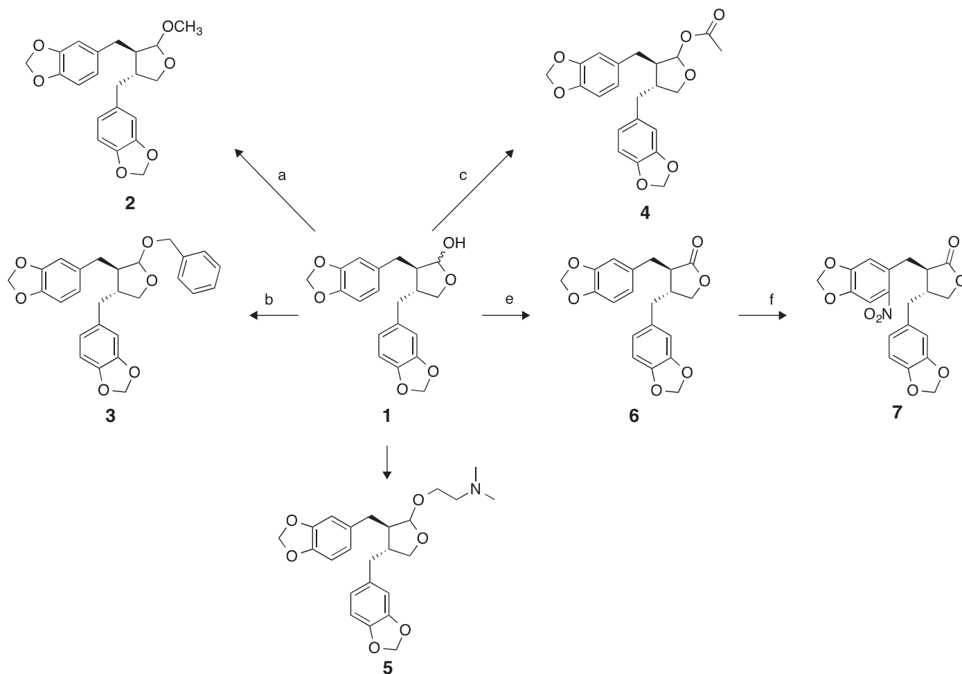
Scheme 1. Obtaining semisynthetic derivatives of 1 : 2 , where: CH 3 I, NaH, dry THF, 30 min, TA atm N 2 ; 3 , where b: benzyl bromide, NaH, THF, 6 h, TA; 4 , where c: acetic anhydride, dry pyridine, toluene, dichloromethane; 5 , where d: dimethylethylamine chloride, sodium ethoxide, reflux for 8 h, 6 where e: PCC, dry DCM, atm N 2 , -60°C, 24 h; 7 , where f: HNO 3 6 equiv, CHCl 3 , 10 °C, 4 h.
