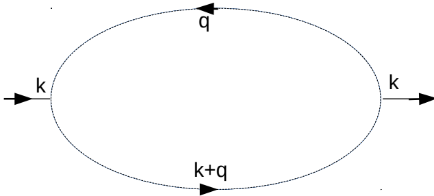
Figure 3: \Pi_2(k) : second order contribution to the trace. The thin lines stand for the propagators D_S . Notice momentum conservation at the vertices.
