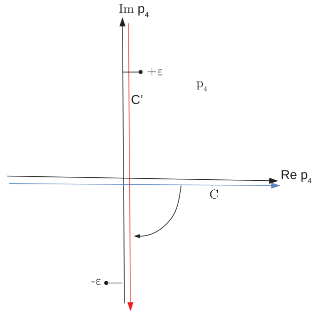
Figure 2: Wick rotation of the blue contour C , running along the real p -axis, into the red contour C' , running along the imaginary p -axis, without crossing the poles. These are shown as blobs, whose distance to the vertical axis is \pm\epsilon .
