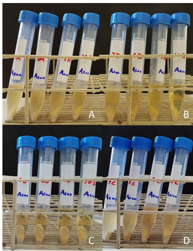
Fig. 3. Roots individually stored in tubes containing brain heart infusion (BHI), showing clear and turbid samples. A – microwave radiation; B – ethylene oxide; C – autoclave; D – control (no sterilization).
