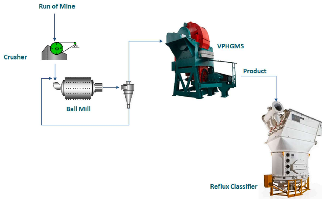
Fig. 7. Re-processing the concentrate from the VPHGMS magnetic separator using the Reflux Classifier.
