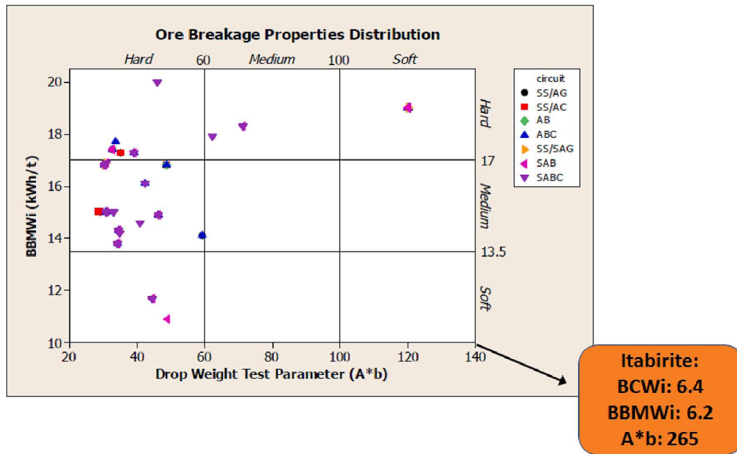
Fig. 8. Values of BWi and A*b from 134 tests in pilot-scale AG/SAG mill (Bueno and Lane, 2011).
