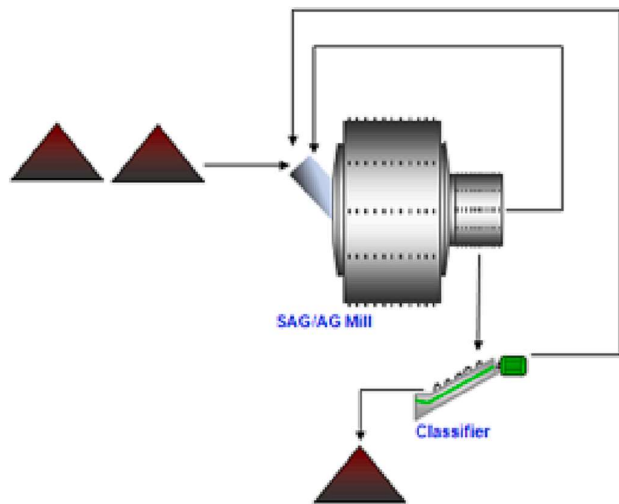
Fig. 3. Circuit configuration of the pilot single stage SAG mill including the spiral classifier (Rodrigues, 2014).
