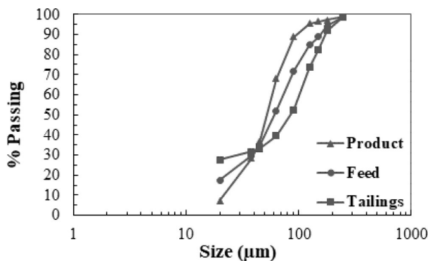
Fig. A2. Size distributions of the three process streams of the pilot scale Reflux Classifier.
