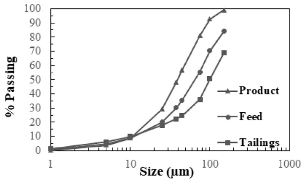
Fig. A1. Size distributions from the pilot-VPHGMS test.
