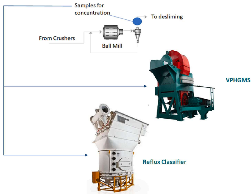
Fig. 4. Source of feed used for the VPHGMS magnetic separator and the Reflux Classifier.
