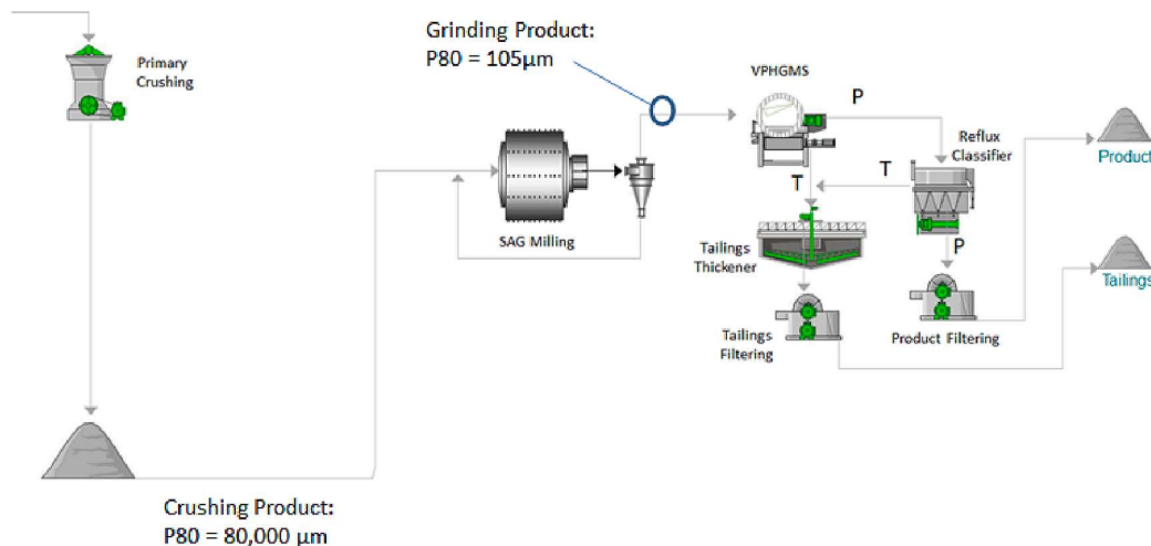
Fig. 2. Proposed disruptive itabirite iron ore circuit.
