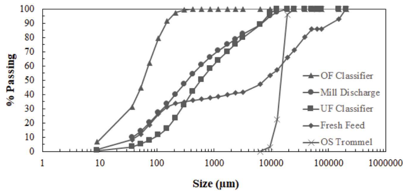
Fig. 9. Size distributions resulting from the pilot-SAG test.
