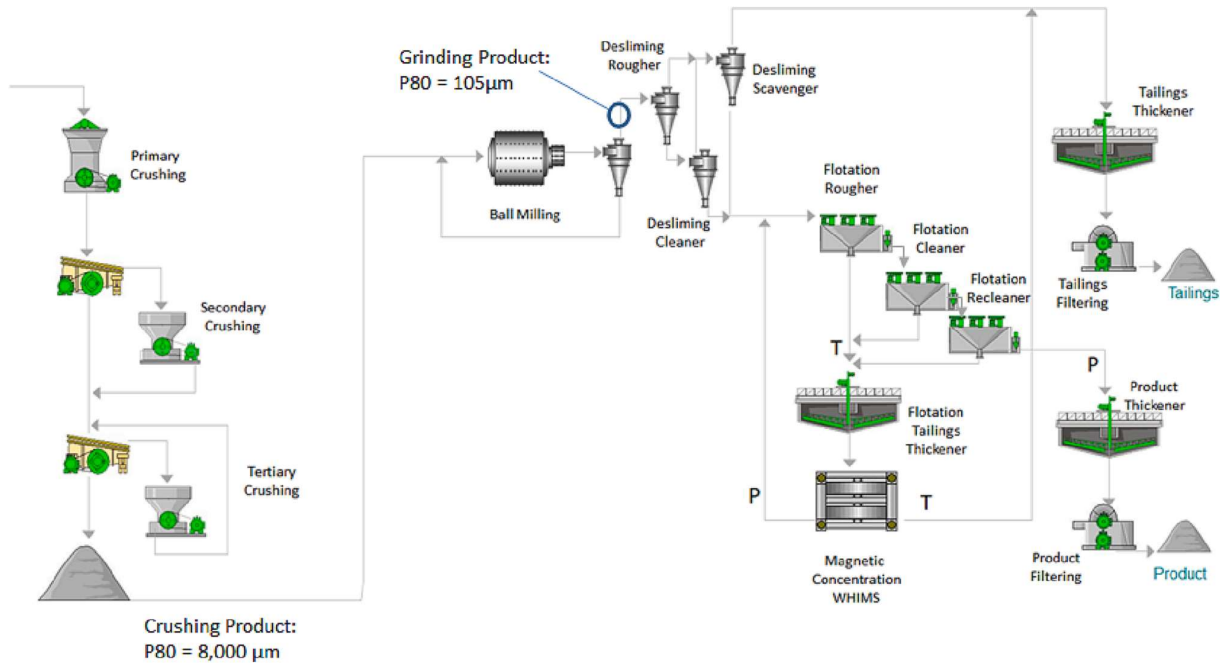
Fig. 1. Conventional itabirite iron ore circuit.
