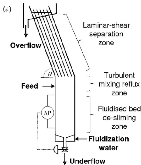
Fig. 6. Schematic representation of the Reflux Classifier (a) and image of the pilot-scale Reflux Classifier (b).
