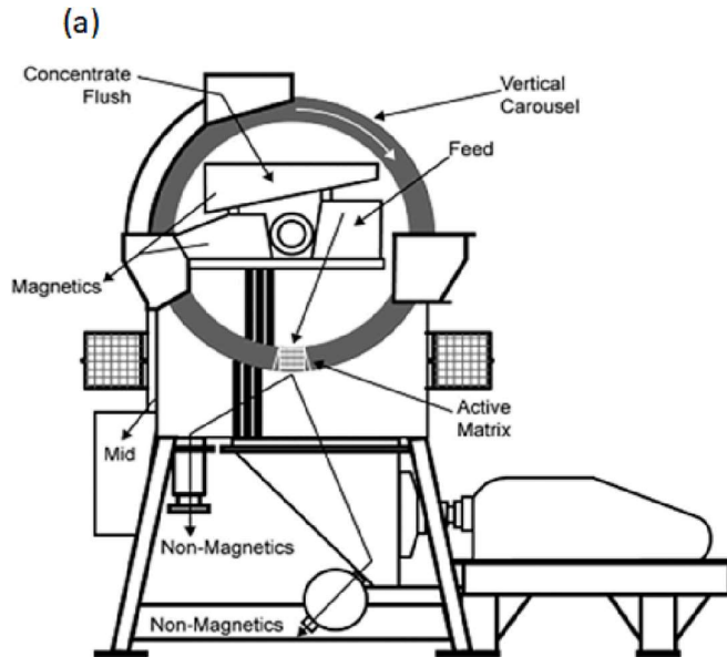
Fig. 5. Schematic representation of the VPHGMS (a) and image of the pilot-scale VPHGMS separator (b).
