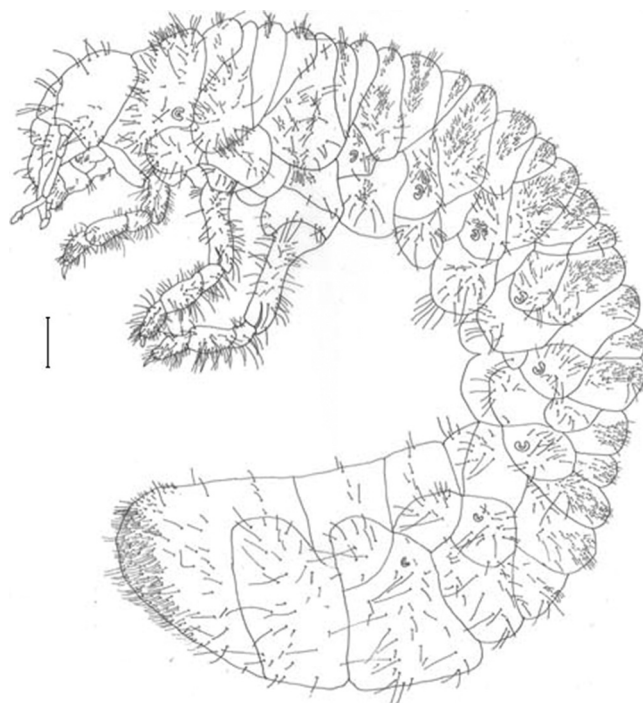
Fig. 1. Larva of the 3rd instar of Liogenys fusca . Scale 1 mm.
