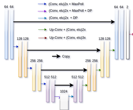
Figure 3: UNet Architecture.
