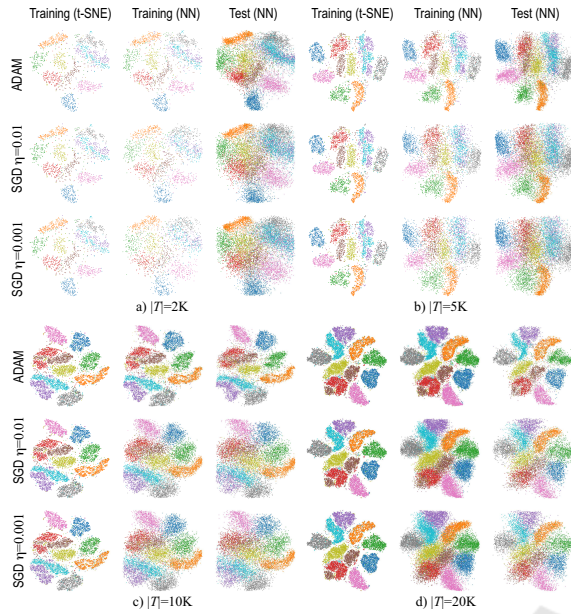
Figure 5: Optimizer: Effects of different settings (ADAM, SGD with \eta \in \{0.001, 0.01\} ) for different training-set sizes. Compare the ground truth (training-set, projected by t-SNE) with the NN results on the training-set, respectively test-set.
