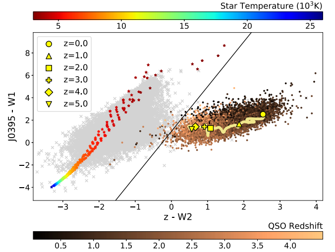
Figure 21. S-PLUS/WISE colour-colour diagram of stars and quasars in the Stripe 82 area from Nakazono et al. (in preparation). Stars with reliable classification in S-PLUS are shown as grey Xs, whereas confirmed quasars (with known spectroscopy) are indicated by circles whose colours depend on the redshift, indicated on the bottom colour bar. Stellar models for different effective temperatures are indicated by star symbols, coloured according to the scale on the top. The yellow curve represents the evolution of the simulated colours for a QSO template with redshift. On top of the curve, the yellow symbols mark the integer values of redshift. The dashed-black line represents an empirical relation (equation 1) to separate stars from quasars. A total of 99.5 per cent of the known quasars in Stripe 82 occupies the expected region in the figure (to the right of the dashed black line), confirming the efficiency of the method.
