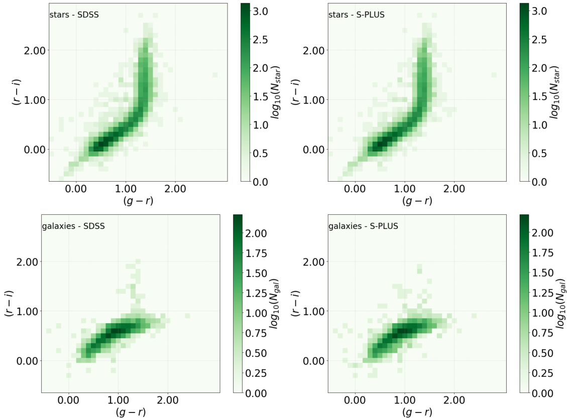
Figure 17. The colour–colour diagram ( g-r ) versus (r-i) using S-PLUS magnitudes down to r = 19 . The overall performance of the code indicates that 97.9 per cent of the objects are correctly classified down to this magnitude limit (see Section 5.1). Upper panels: The stellar locus of objects classified as stars based on SDSS (left) and S-PLUS (right) data. Lower panel: The galaxy locus in the same diagram using the SDSS and S-PLUS classifications.
