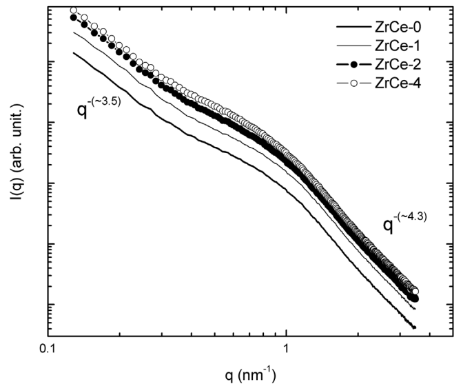
Fig. 5. Small angle X-ray scattering of bare ZrCe samples showing two ranges of scattering angle behavior.
