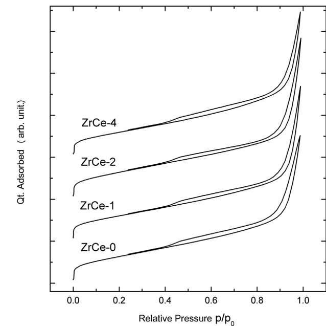
Fig. 3. Nitrogen Adsorption Isotherms of bare ZrCe samples showing the slit like mesoporous type of hysteresis loop.
